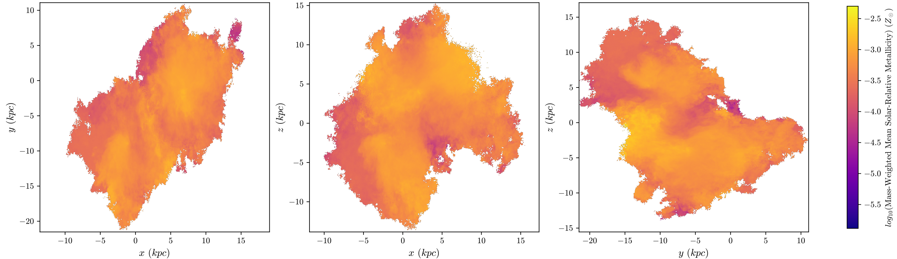
T1 Aug Mass-Weighted Mean Metallicity, z = 2.494 , 512 bins
