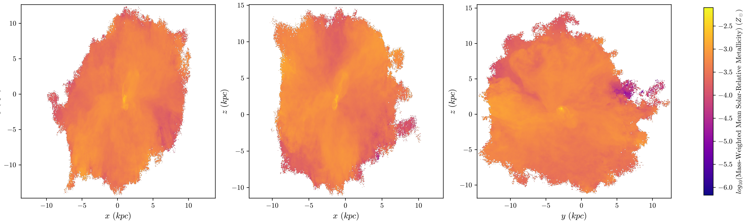
T1 Aug Mass-Weighted Mean Metallicity, z = 2.208 , 512 bins
