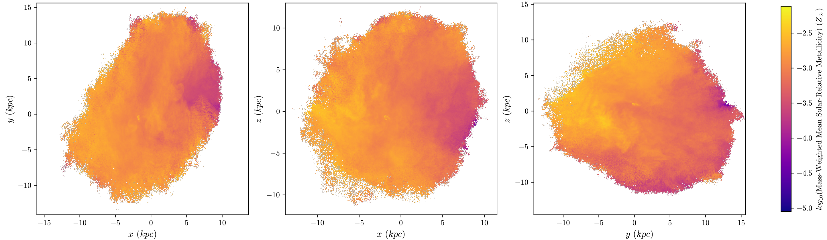
T1 Aug Mass-Weighted Mean Metallicity, z = 1.96 , 512 bins
