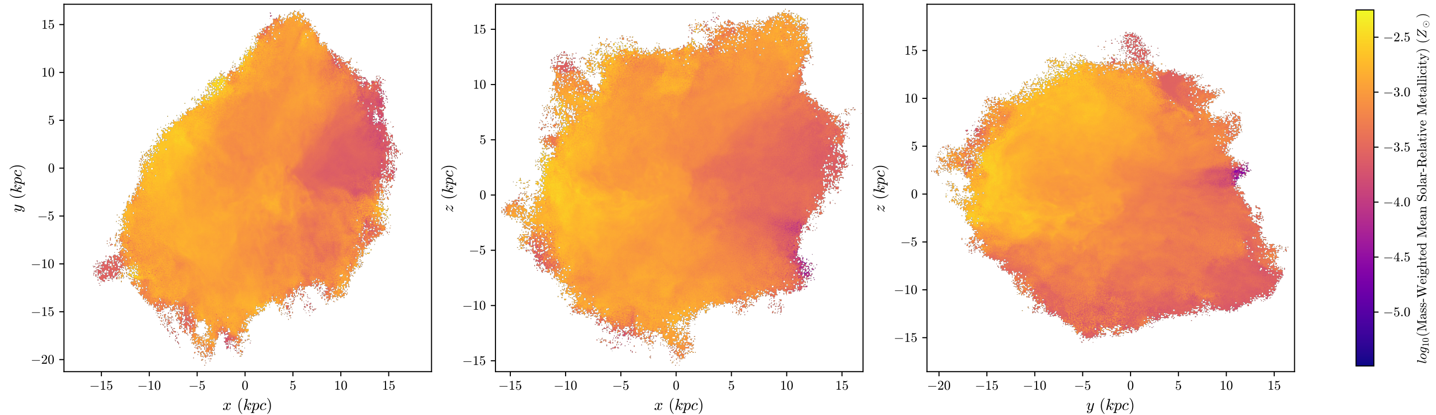
T1 Aug Mass-Weighted Mean Metallicity, z = 1.77 , 512 bins
