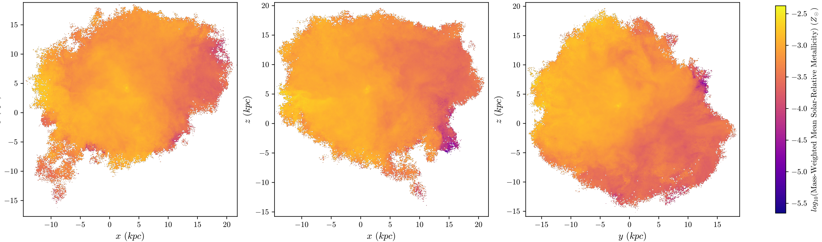
T1 Aug Mass-Weighted Mean Metallicity, z = 1.449 , 512 bins
