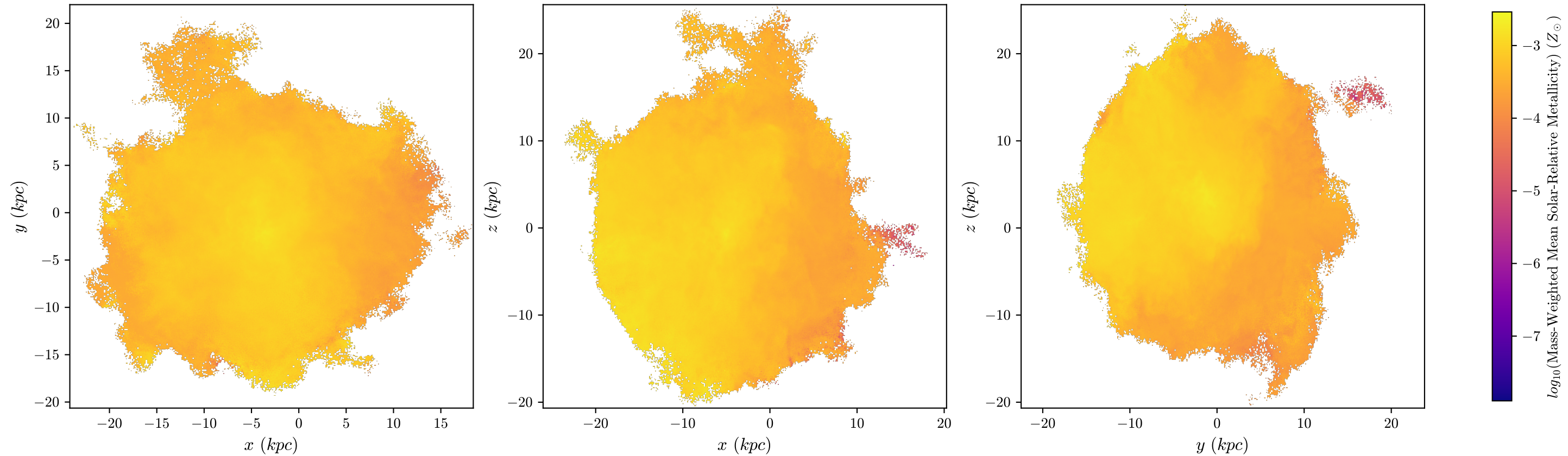
T1 Aug Mass-Weighted Mean Metallicity, z = 1.094 , 512 bins
