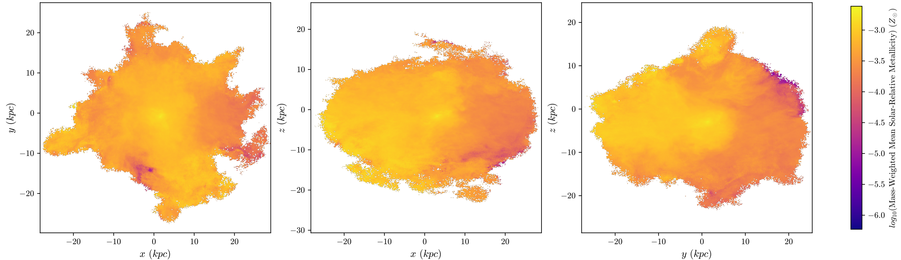
T1 Aug Mass-Weighted Mean Metallicity, z = 0.914 , 512 bins
