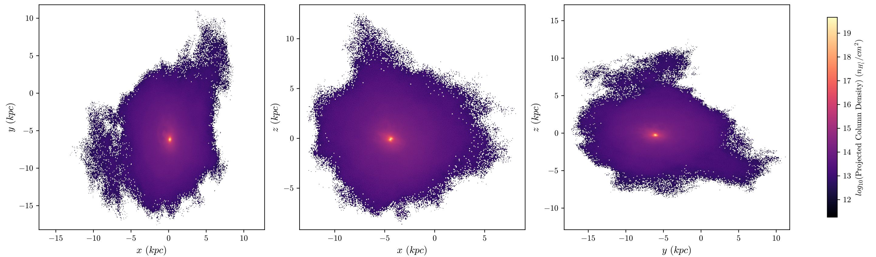
T4 Aug Neutral Hydrogen Fraction, z = 2.208 , 512 bins
