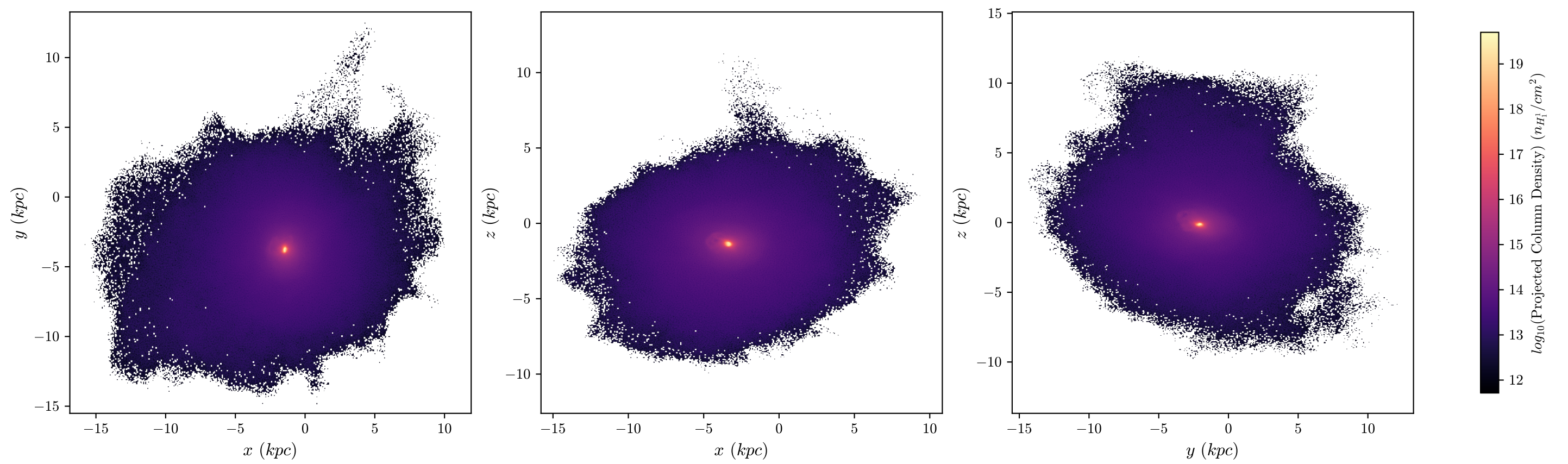
T4 Aug Neutral Hydrogen Fraction, z = 1.77 , 512 bins
