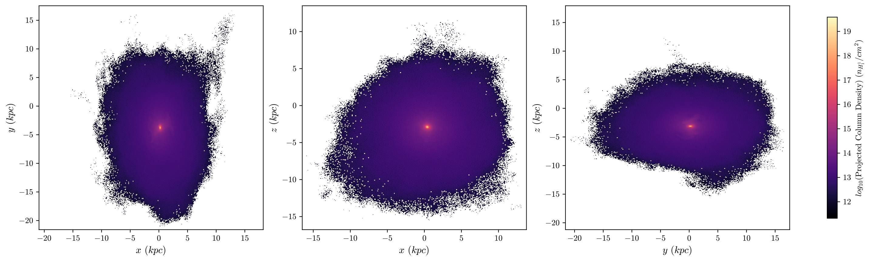
T4 Aug Neutral Hydrogen Fraction, z = 1.196 , 512 bins
