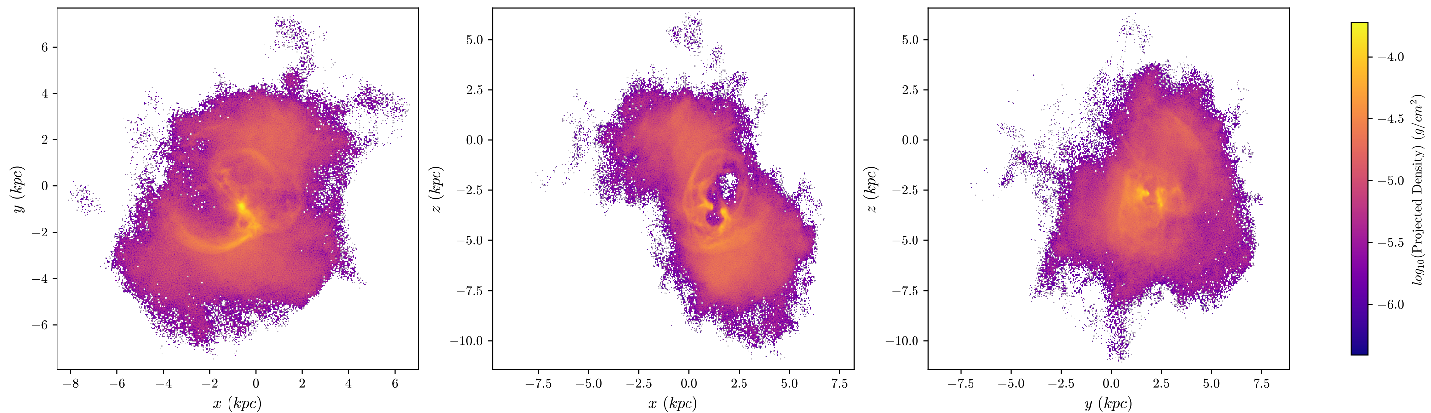
T4 Aug Dark Matter, z = 4.008 , 512 bins
