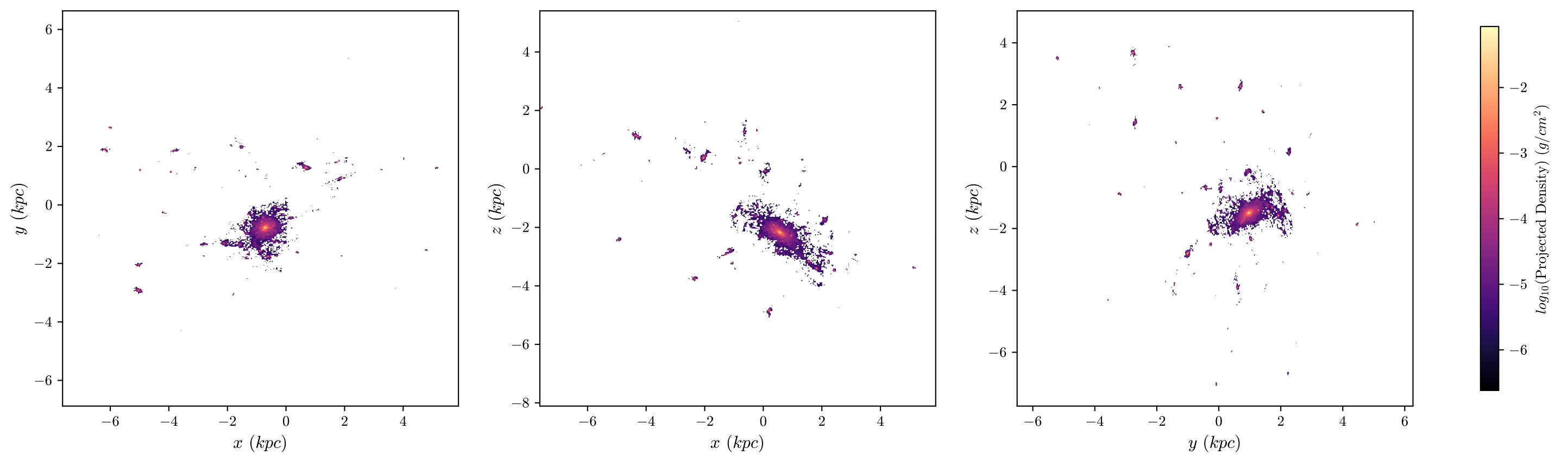
T4 Aug Stars, z = 4.008 , 512 bins
