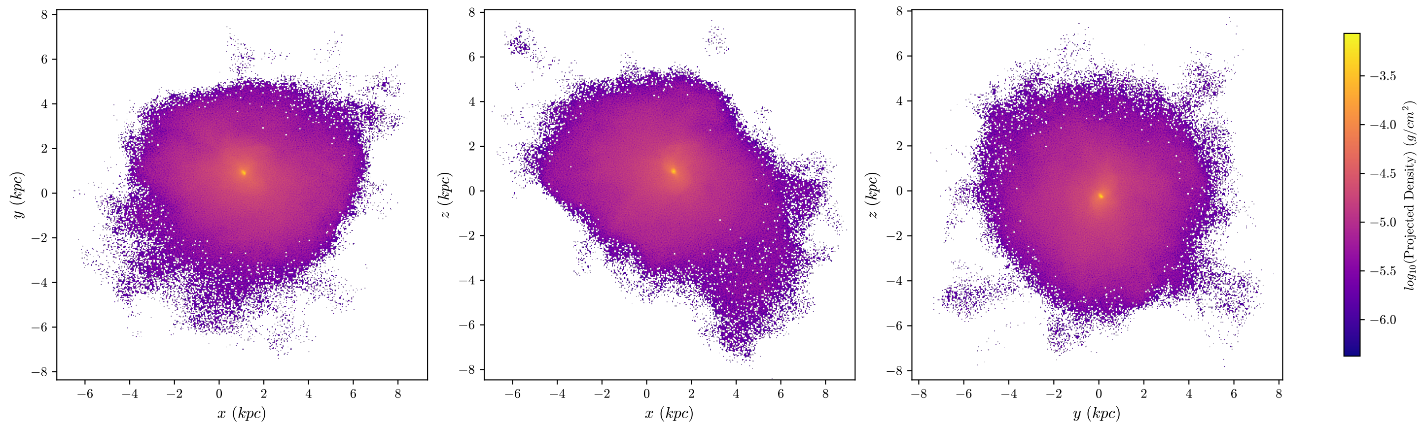
T4 Aug Dark Matter, z = 3.344 , 512 bins
