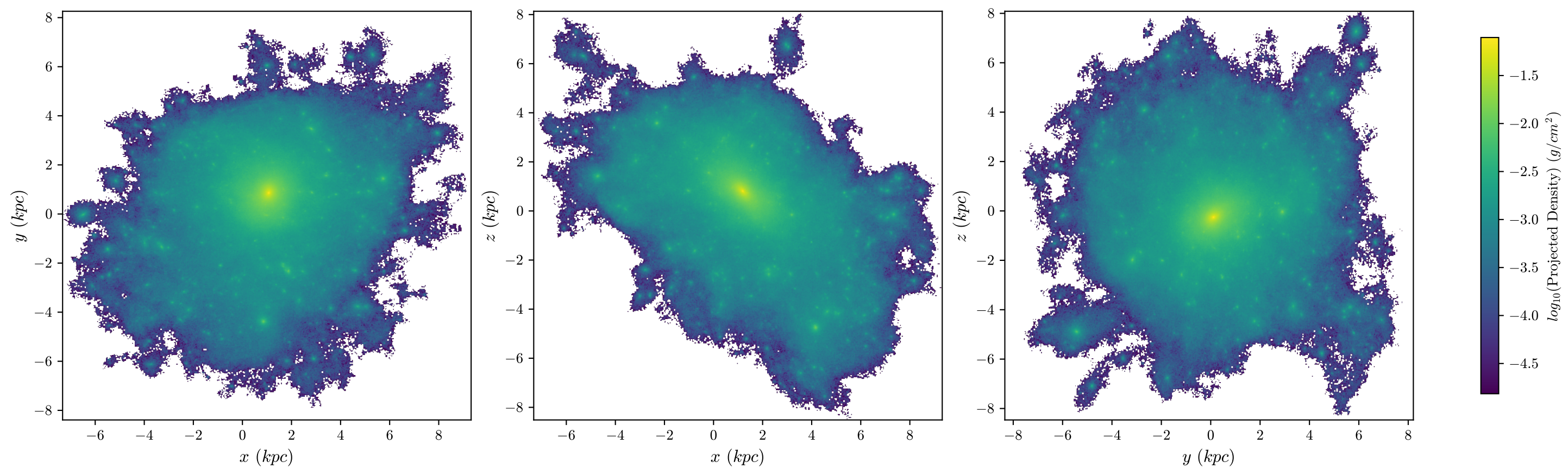
T4 Aug Stars, z = 3.344 , 512 bins
