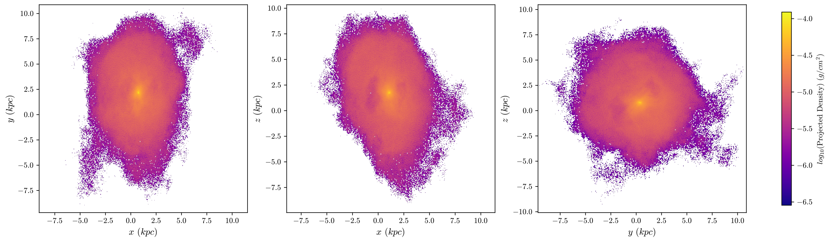
T4 Aug Dark Matter, z = 2.859 , 512 bins
