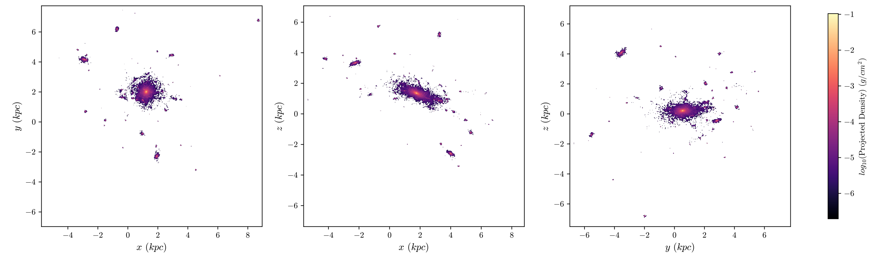
T4 Aug Stars, z = 2.859 , 512 bins
