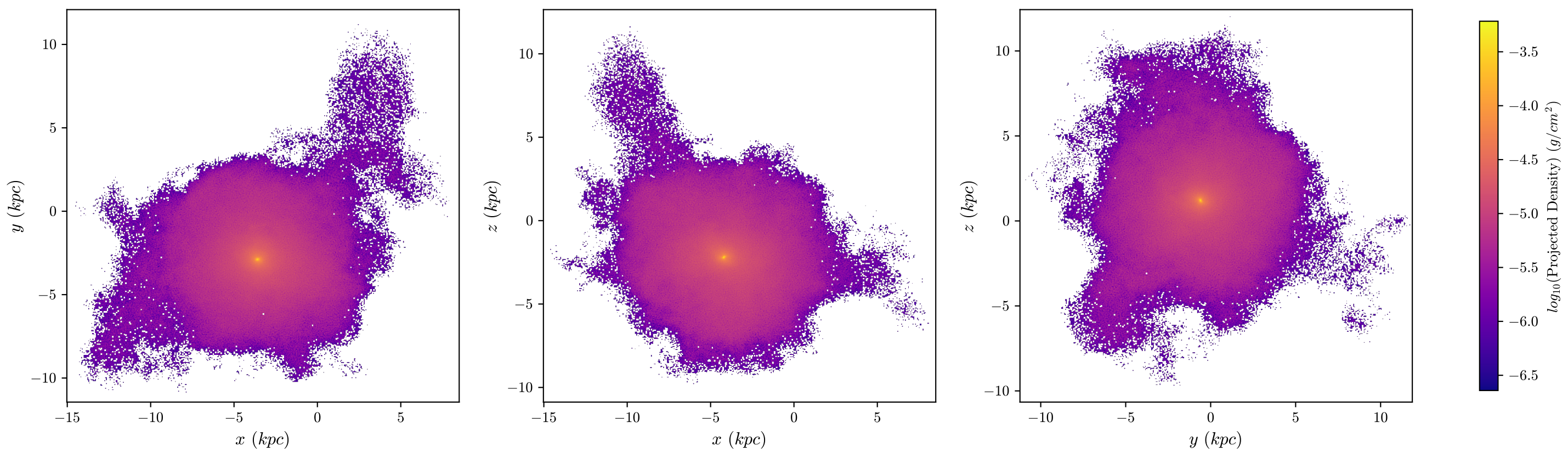
T4 Aug Dark Matter, z = 2.494 , 512 bins
