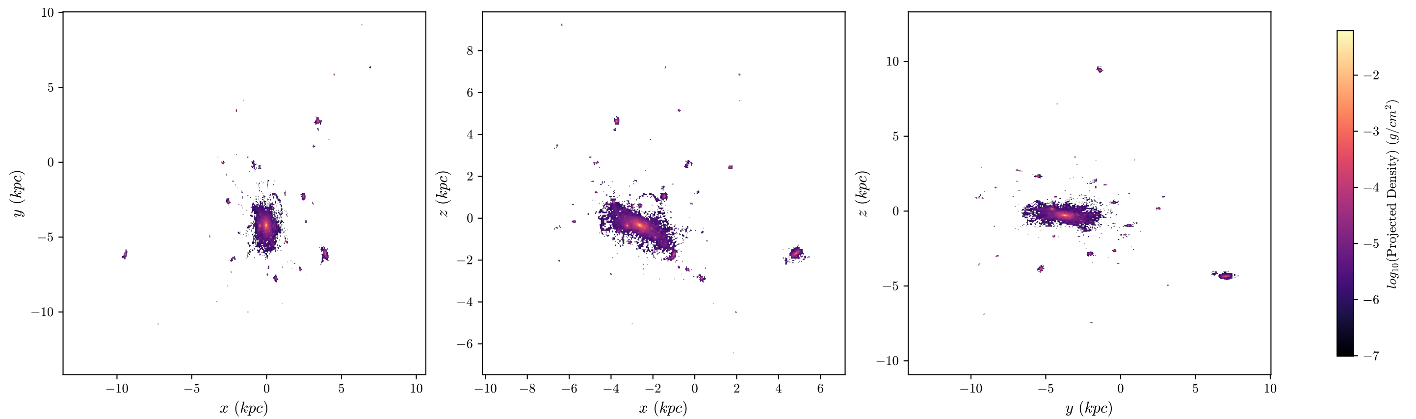
T4 Aug Stars, z = 2.208 , 512 bins
