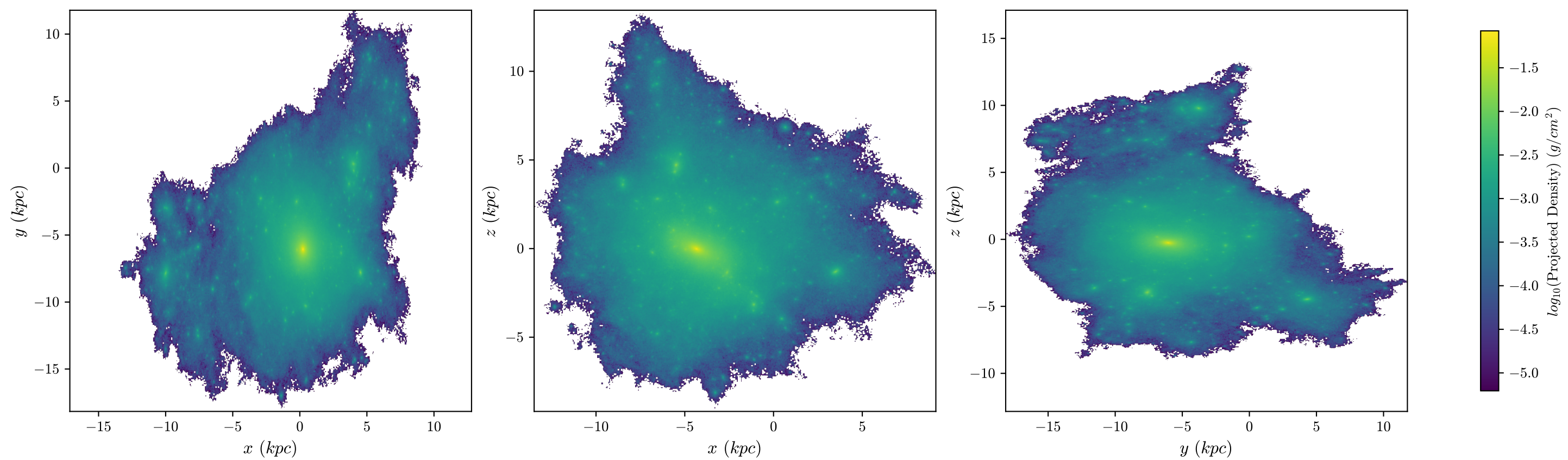
T4 Aug Stars, z = 2.208 , 512 bins
