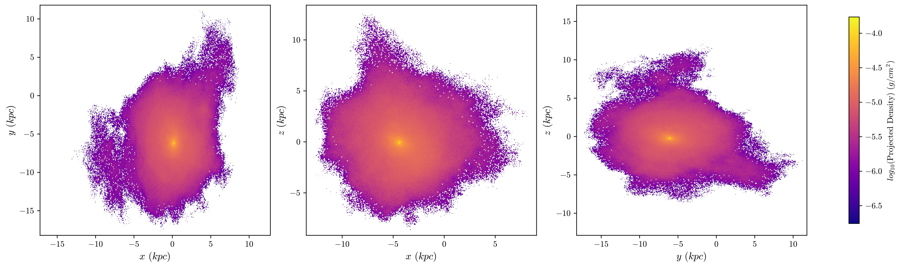
T4 Aug Dark Matter, z = 2.208 , 512 bins
