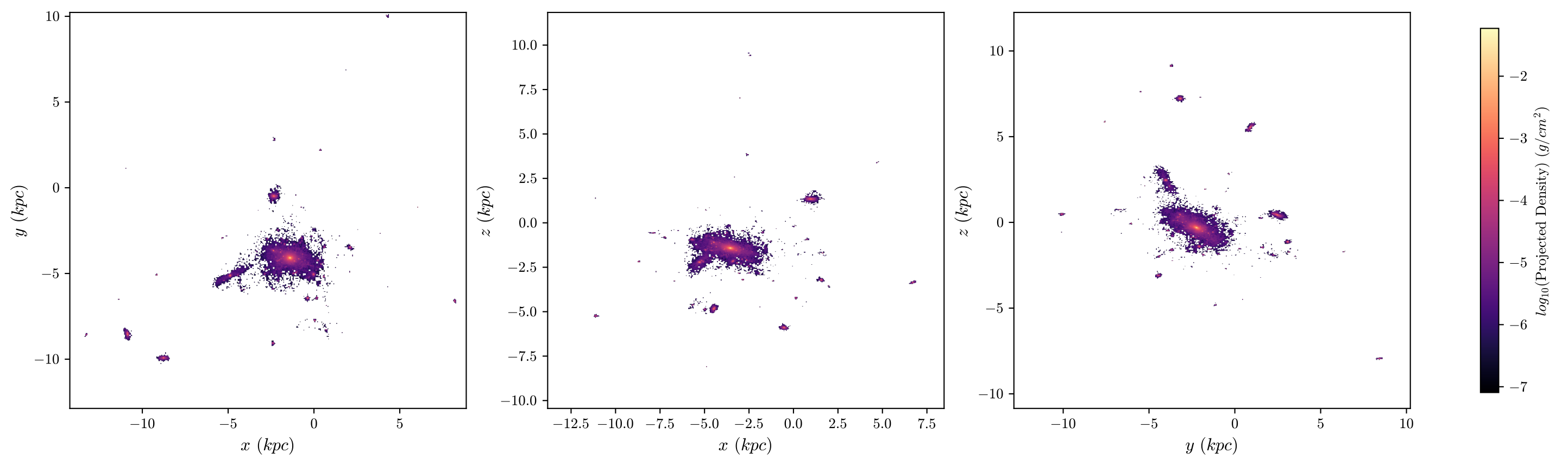
T4 Aug Stars, z = 1.77 , 512 bins
