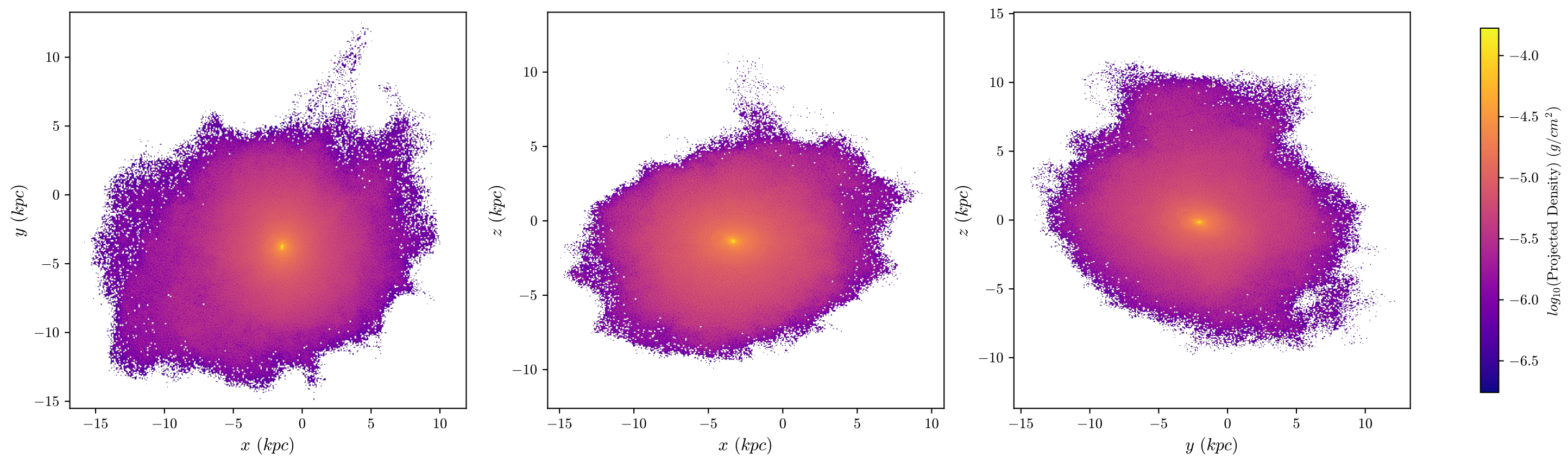
T4 Aug Dark Matter, z = 1.77 , 512 bins
