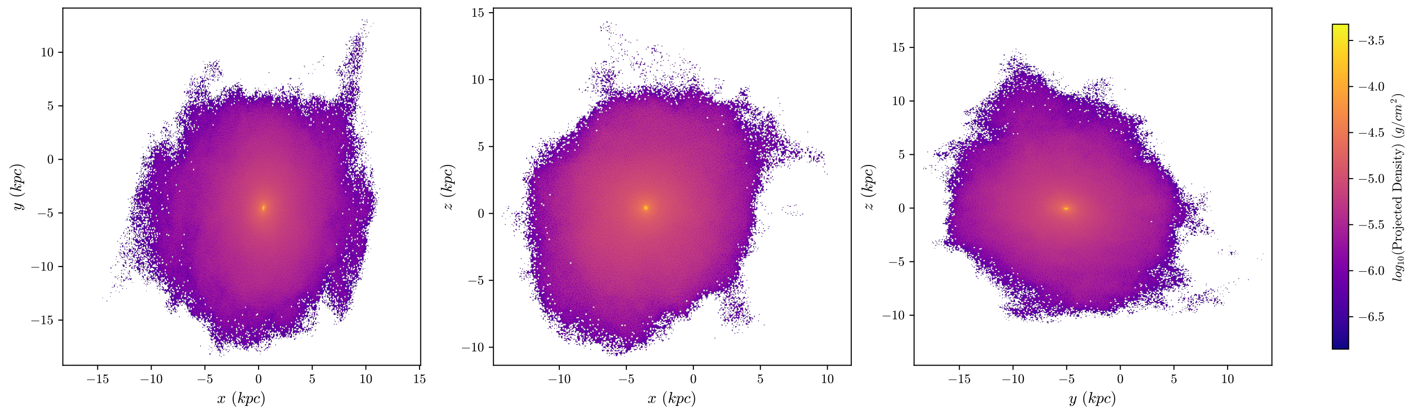
T4 Aug Dark Matter, z = 1.592 , 512 bins
