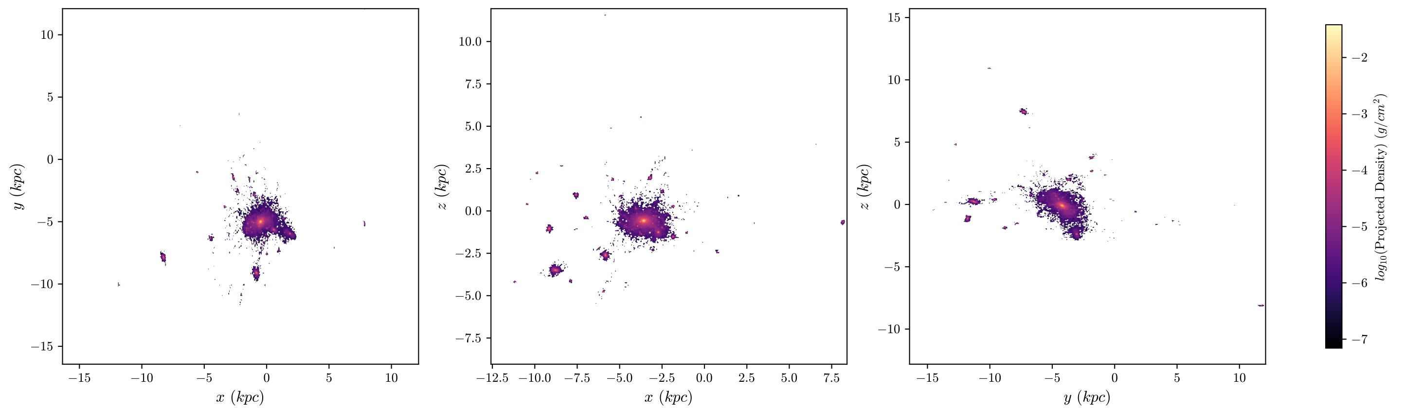
T4 Aug Stars, z = 1.592 , 512 bins
