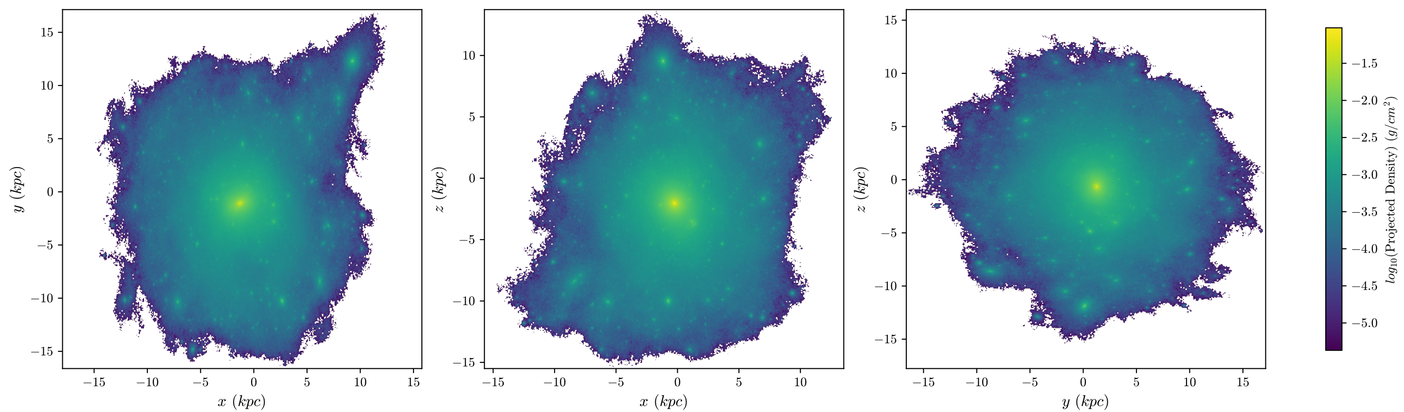
T4 Aug Stars, z = 1.313 , 512 bins
