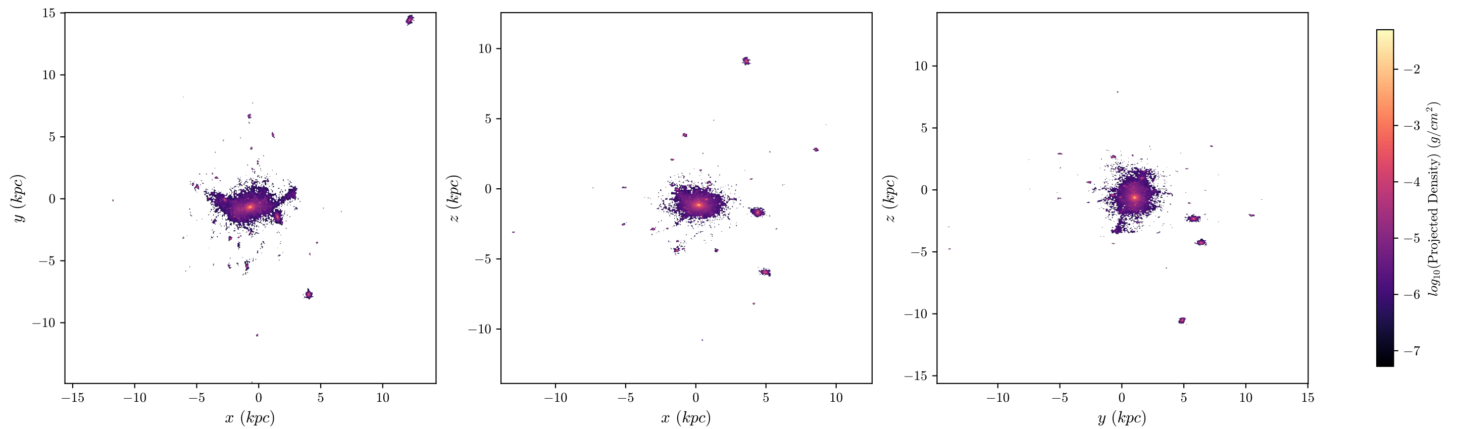
T4 Aug Stars, z = 1.196 , 512 bins
