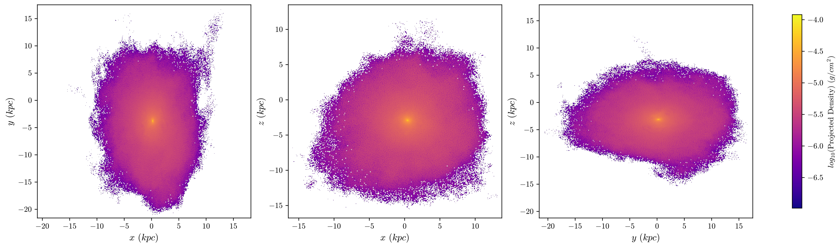
T4 Aug Dark Matter, z = 1.196 , 512 bins
