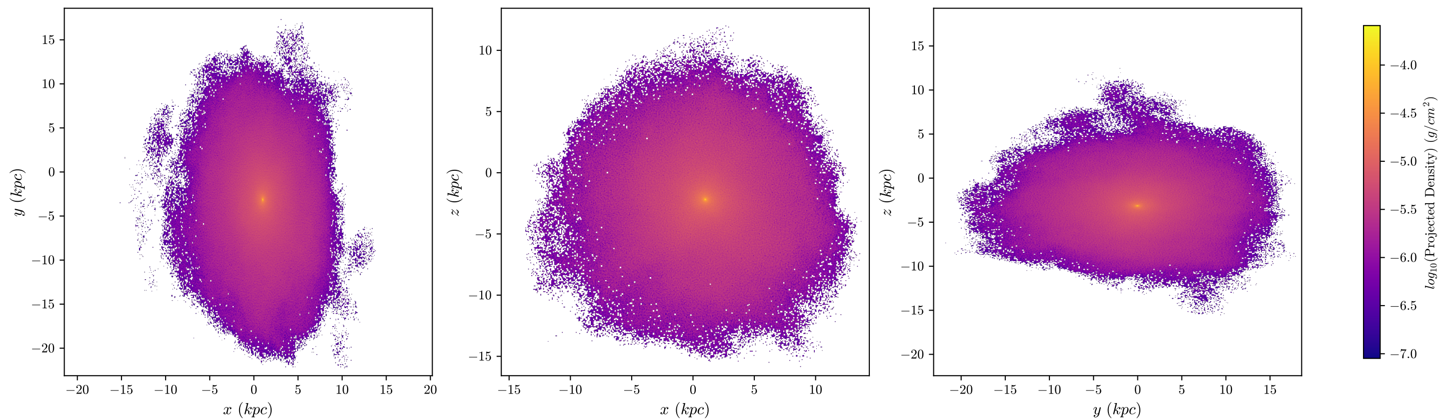
T4 Aug Dark Matter, z = 1.094 , 512 bins
