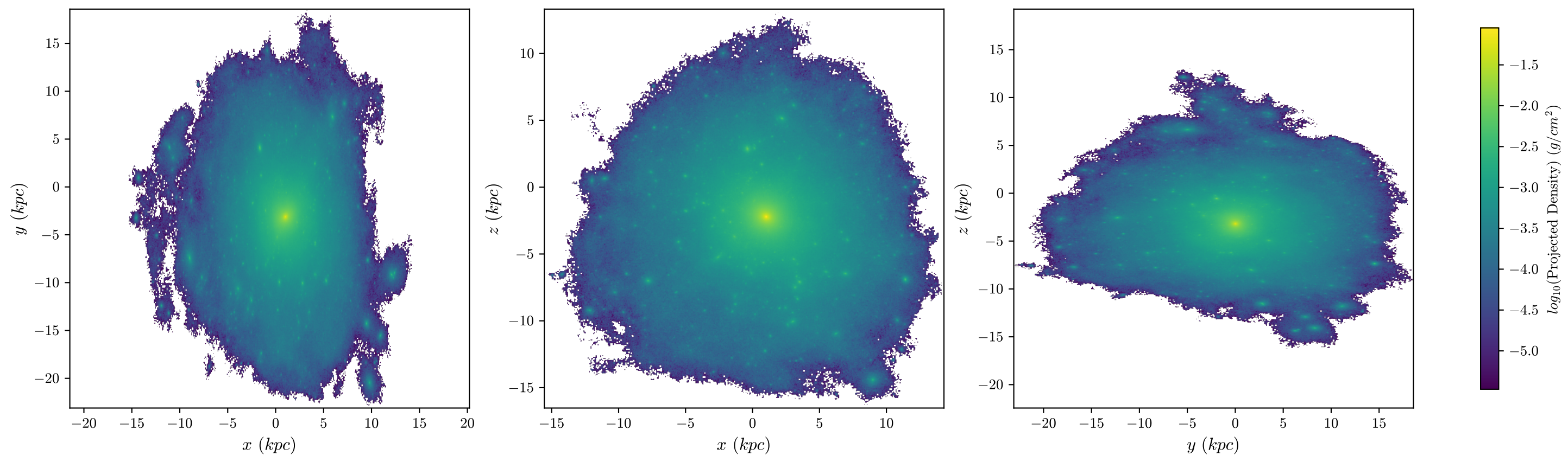
T4 Aug Stars, z = 1.094 , 512 bins
