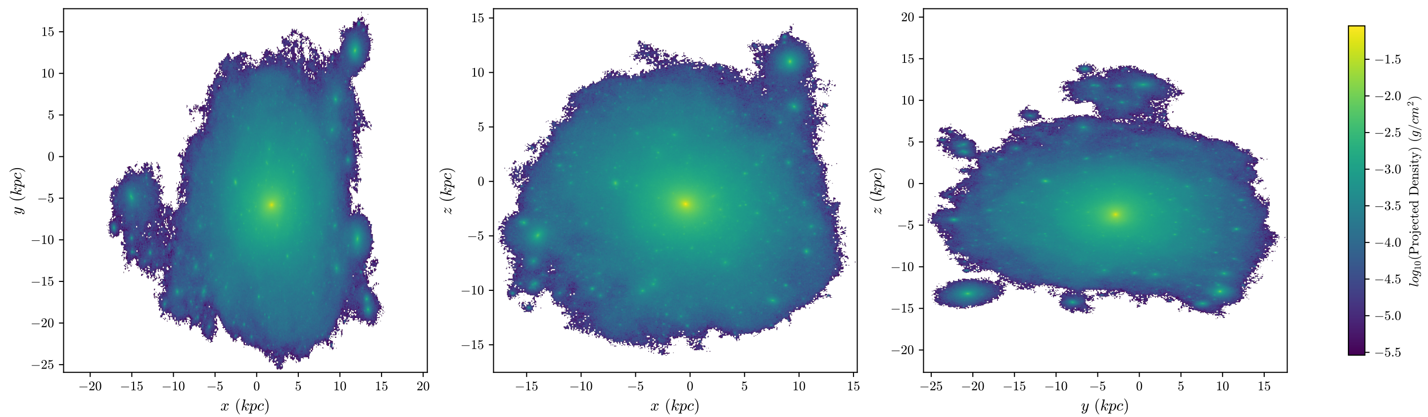
T4 Aug Stars, z = 0.997 , 512 bins
