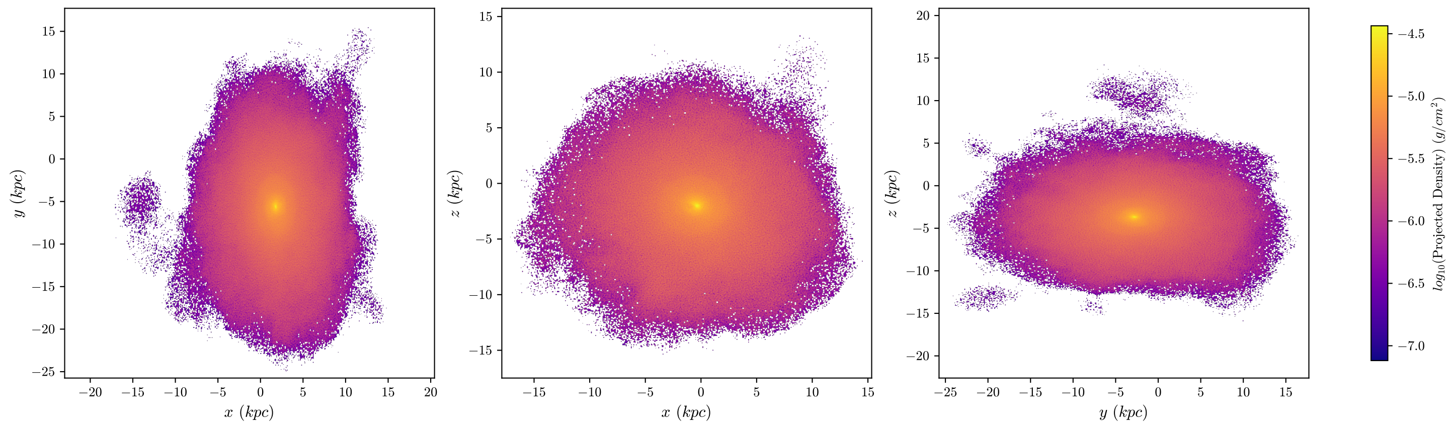
T4 Aug Dark Matter, z = 0.997 , 512 bins
