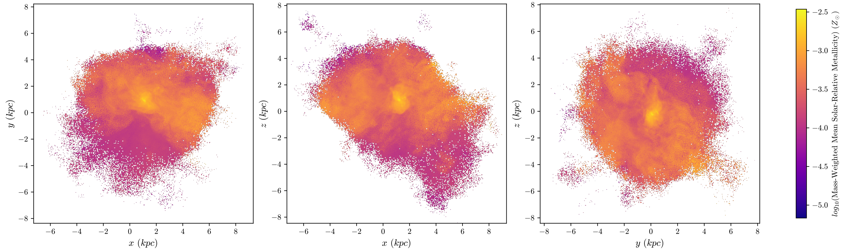
T4 Aug Mass-Weighted Mean Metallicity, z = 3.344 , 512 bins
