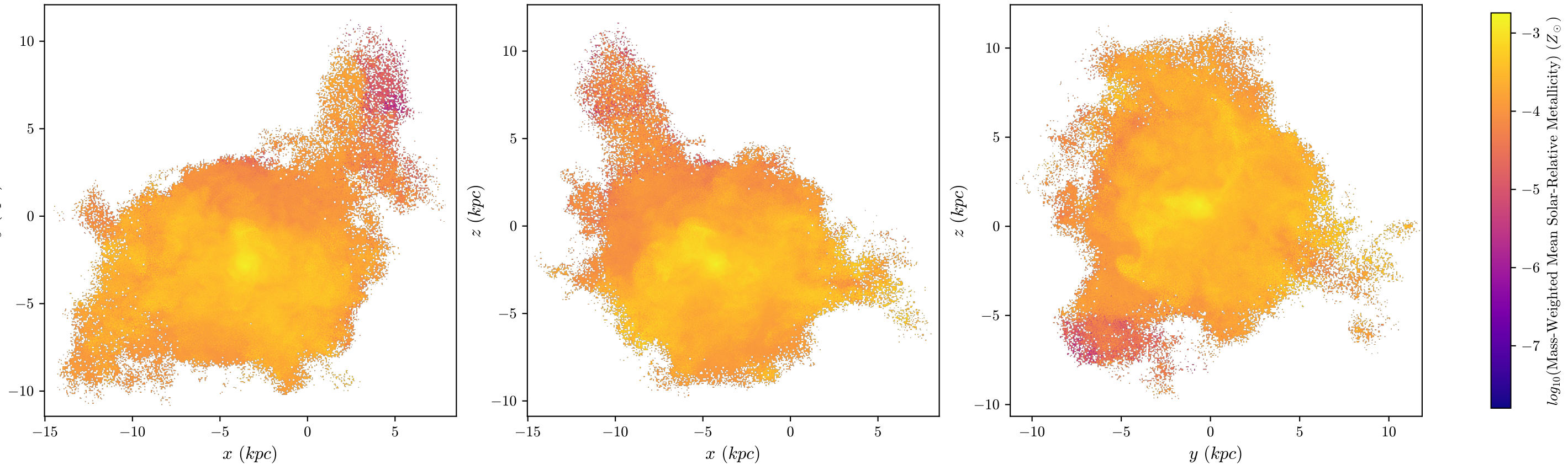
T4 Aug Mass-Weighted Mean Metallicity, z = 2.494 , 512 bins
