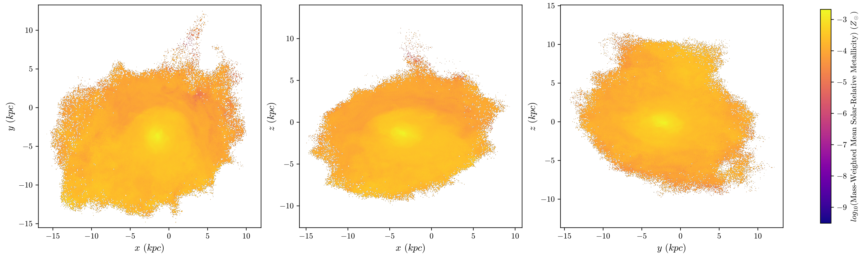
T4 Aug Mass-Weighted Mean Metallicity, z=1.77 , 512 bins
