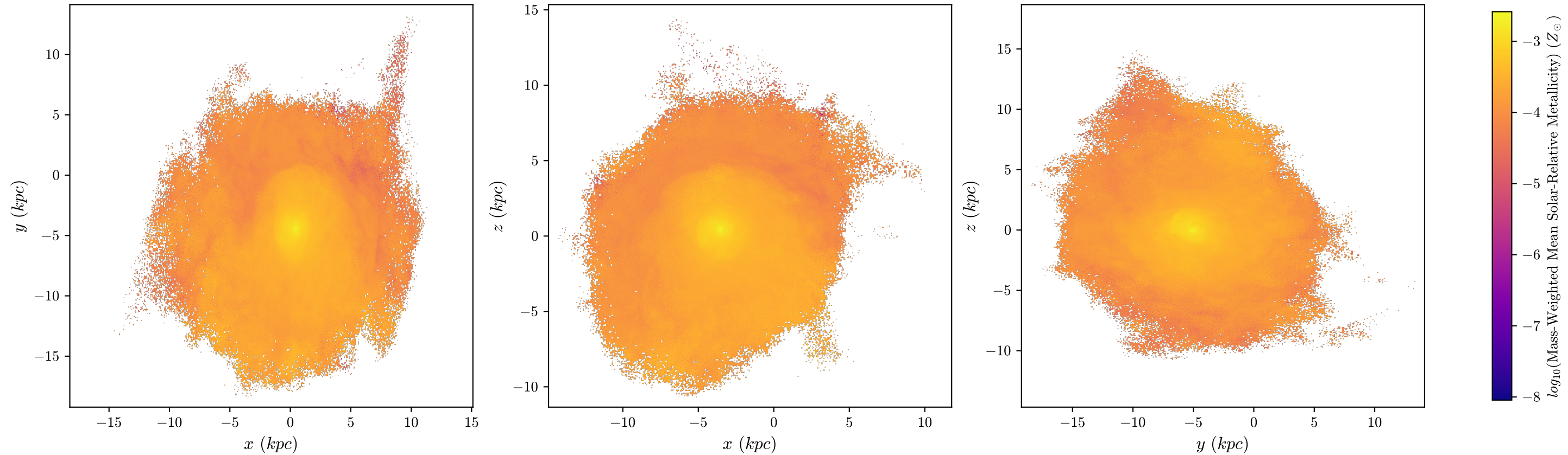
T4 Aug Mass-Weighted Mean Metallicity, z = 1.592 , 512 bins
