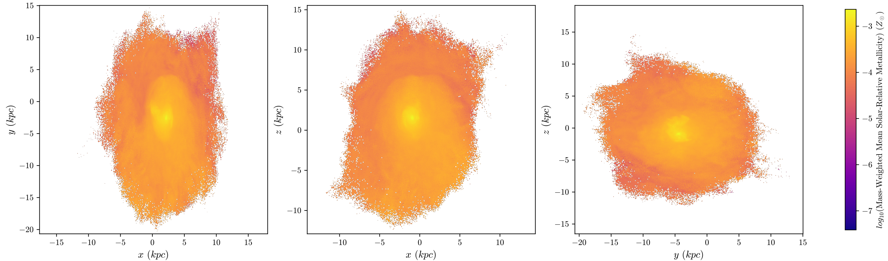
T4 Aug Mass-Weighted Mean Metallicity, z = 1.449 , 512 bins
