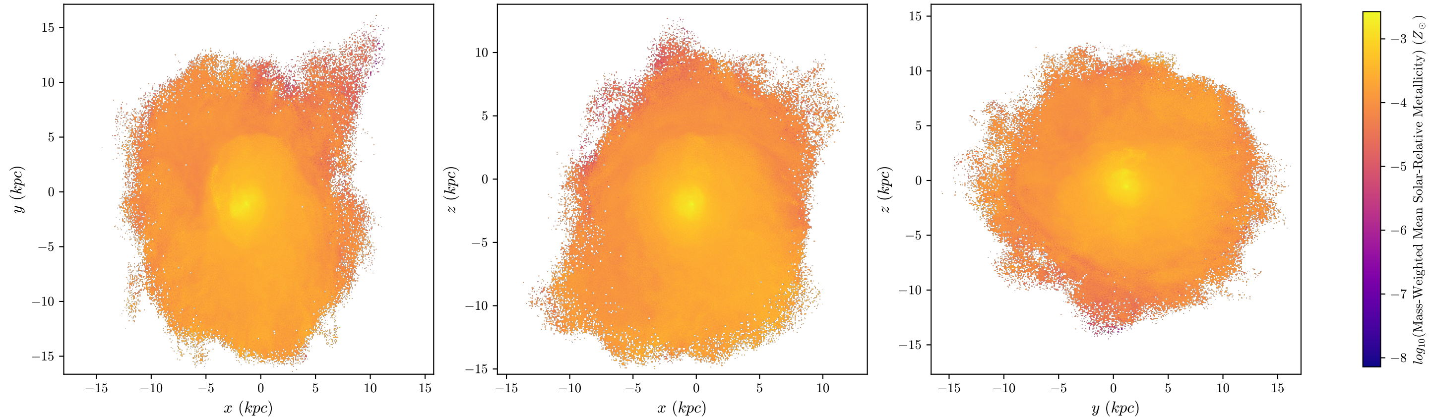
T4 Aug Mass-Weighted Mean Metallicity, z = 1.313 , 512 bins
