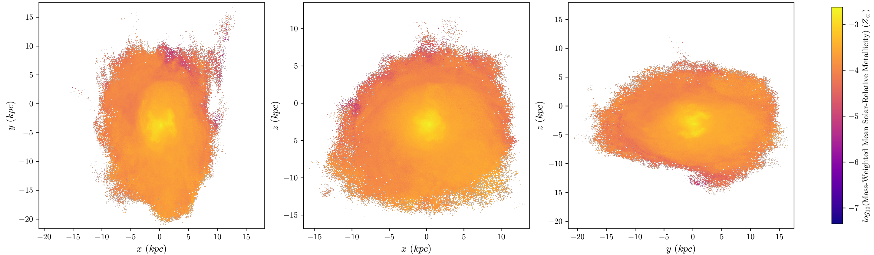
T4 Aug Mass-Weighted Mean Metallicity, z = 1.196 , 512 bins
