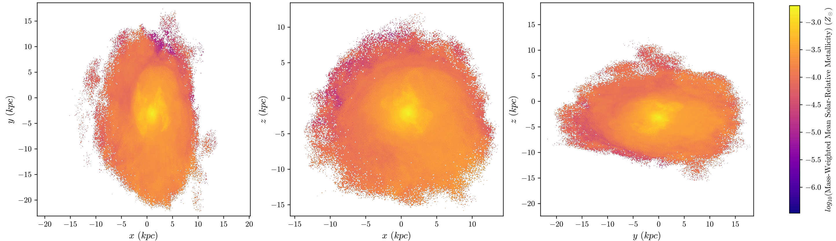
T4 Aug Mass-Weighted Mean Metallicity, z = 1.094 , 512 bins
