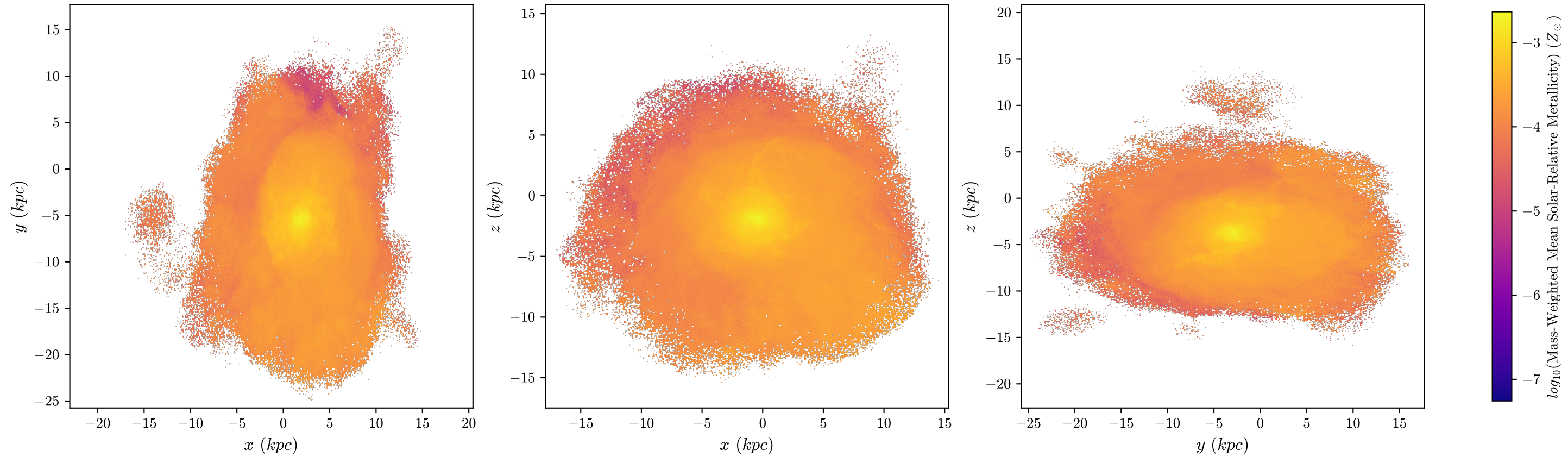
T4 Aug Mass-Weighted Mean Metallicity, z = 0.997 , 512 bins
