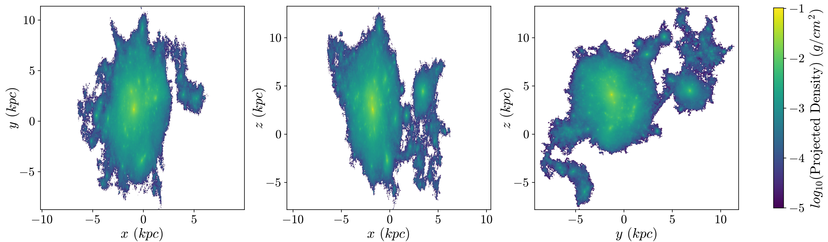
T1 Aug Stars, z = 4.008 , 512px
