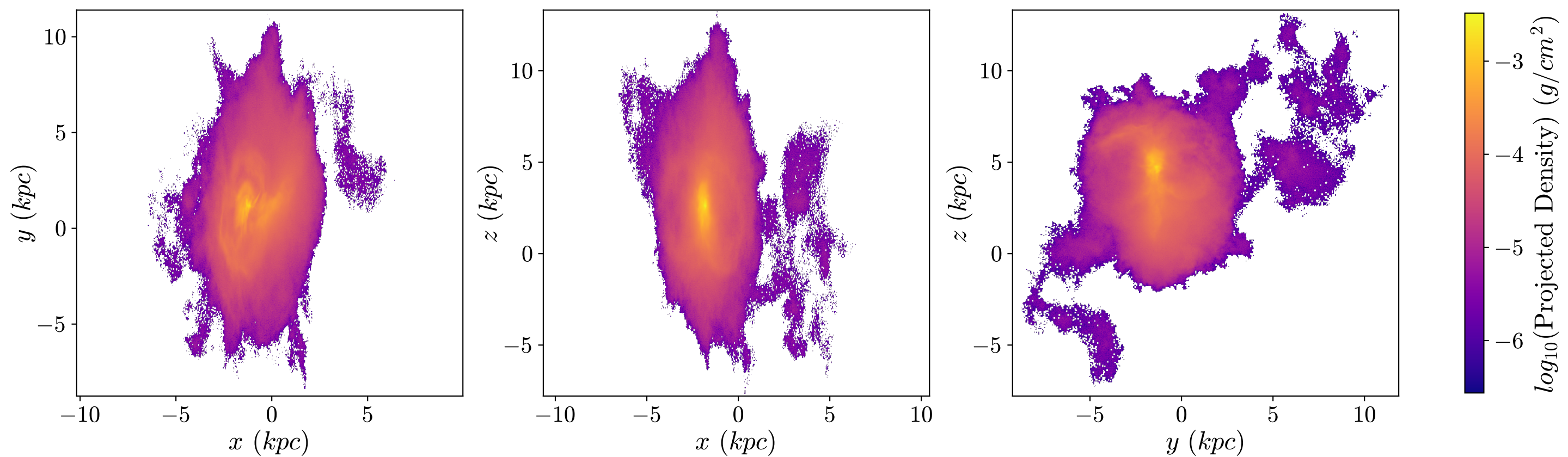
T1 Aug Dark Matter, z = 4.008 , 512px
