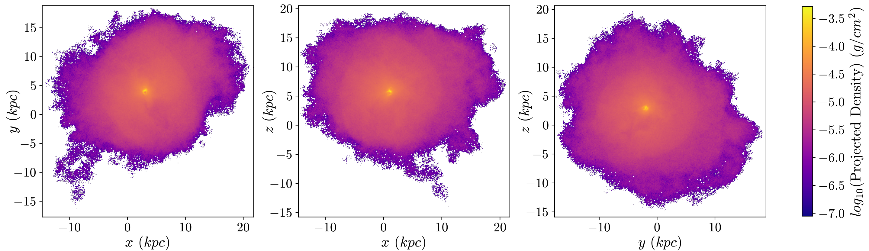
T1 Aug Dark Matter, z = 1.449 , 512px
