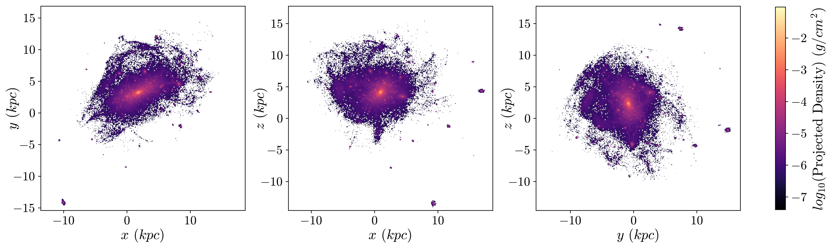
T1 Aug Stars, z = 1.449 , 512px
