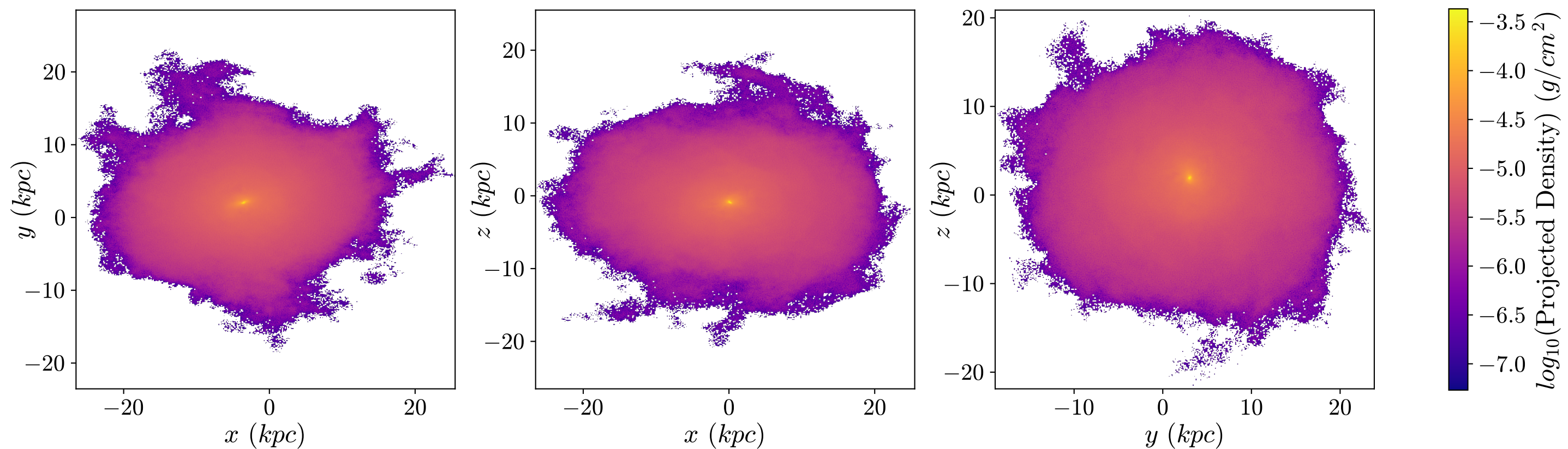
T1 Aug Dark Matter, z = 0.997 , 512px
