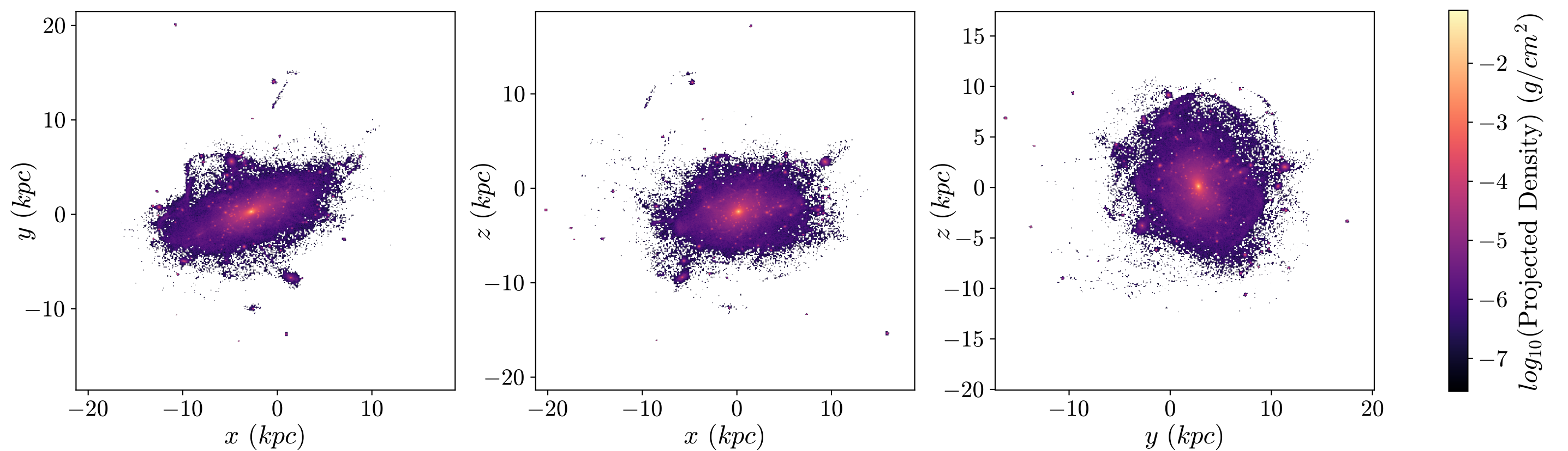
T1 Aug Stars, z = 0.997 , 512px
