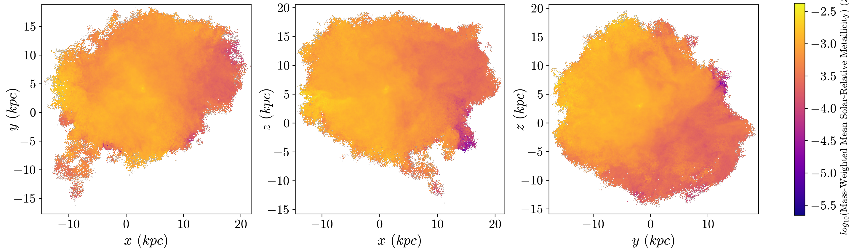
T1 Aug Mass-Weighted Mean Metallicity, z = 1.449 , 512 bins
