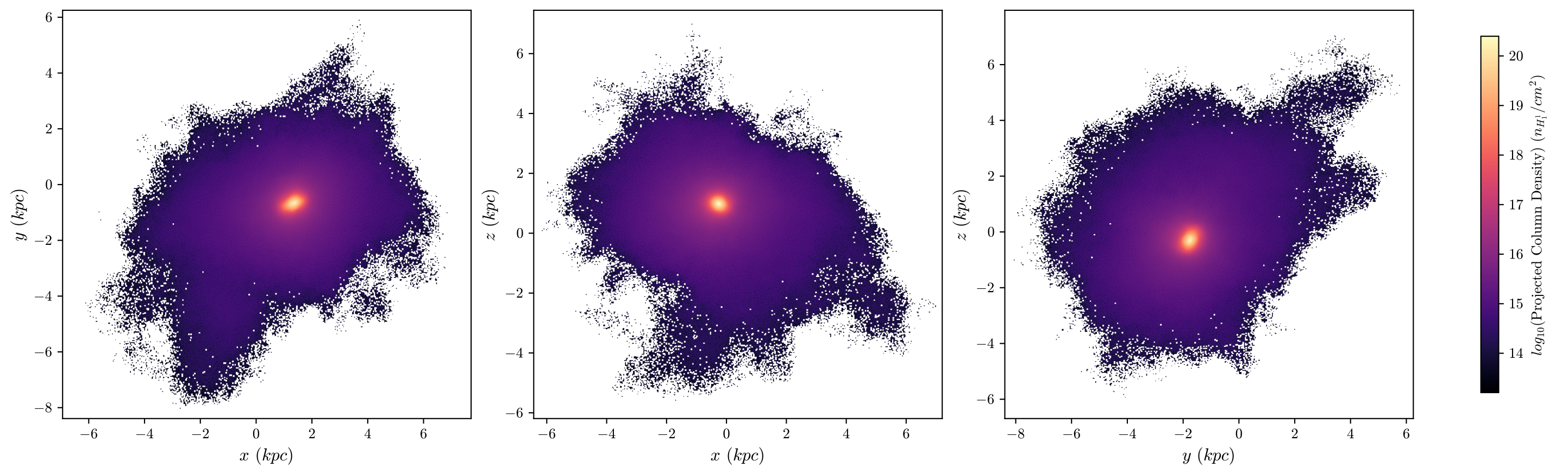
halo8 Neutral Hydrogen Fraction, z = 3.687 , 512 bins
