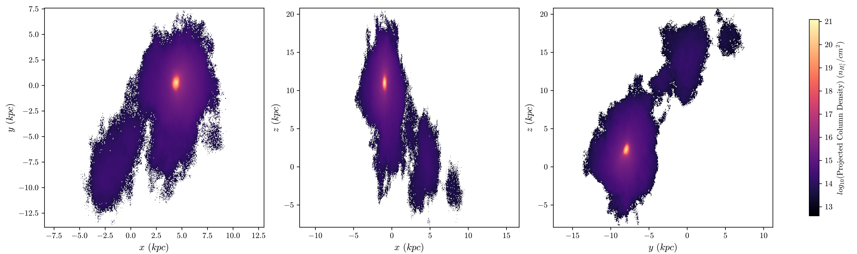
halo8 Neutral Hydrogen Fraction, z = 3.386 , 512 bins
