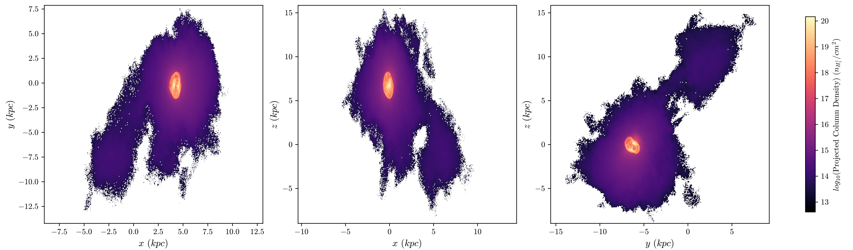
halo8 Neutral Hydrogen Fraction, z = 3.263 , 512 bins
