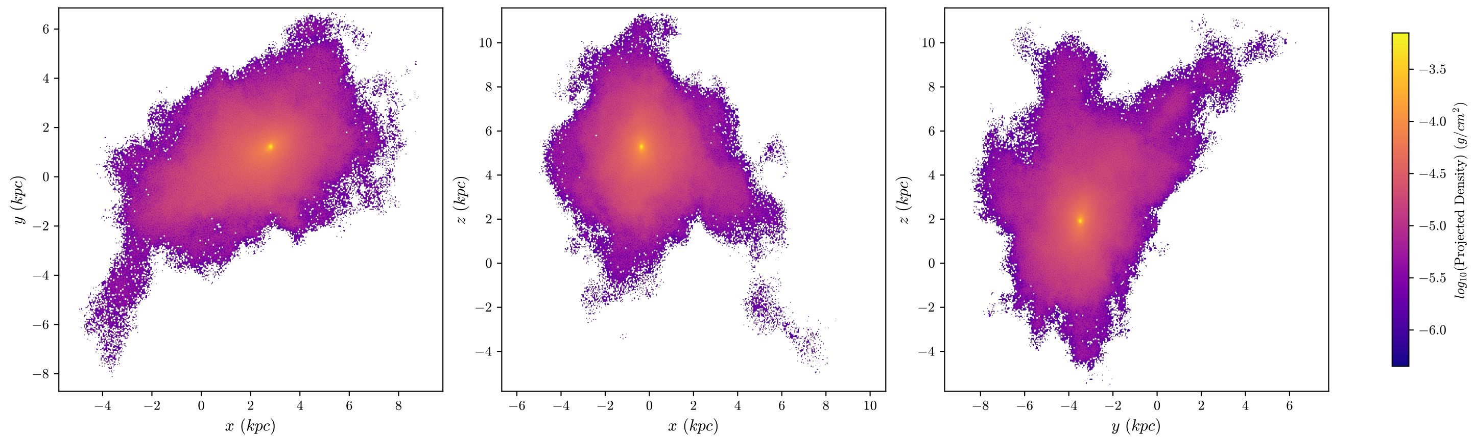
halo8 Dark Matter, z = 3.984 , 512 bins
