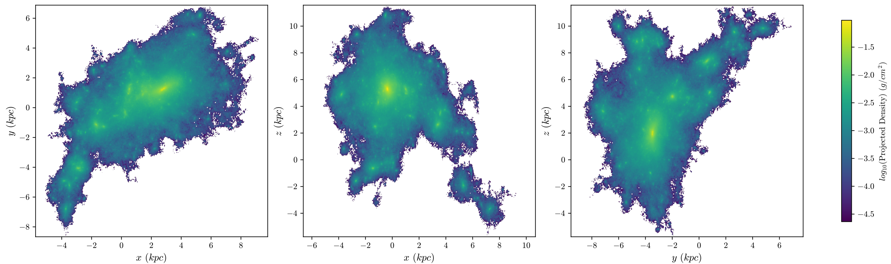
halo8 Stars, z = 3.984 , 512 bins
