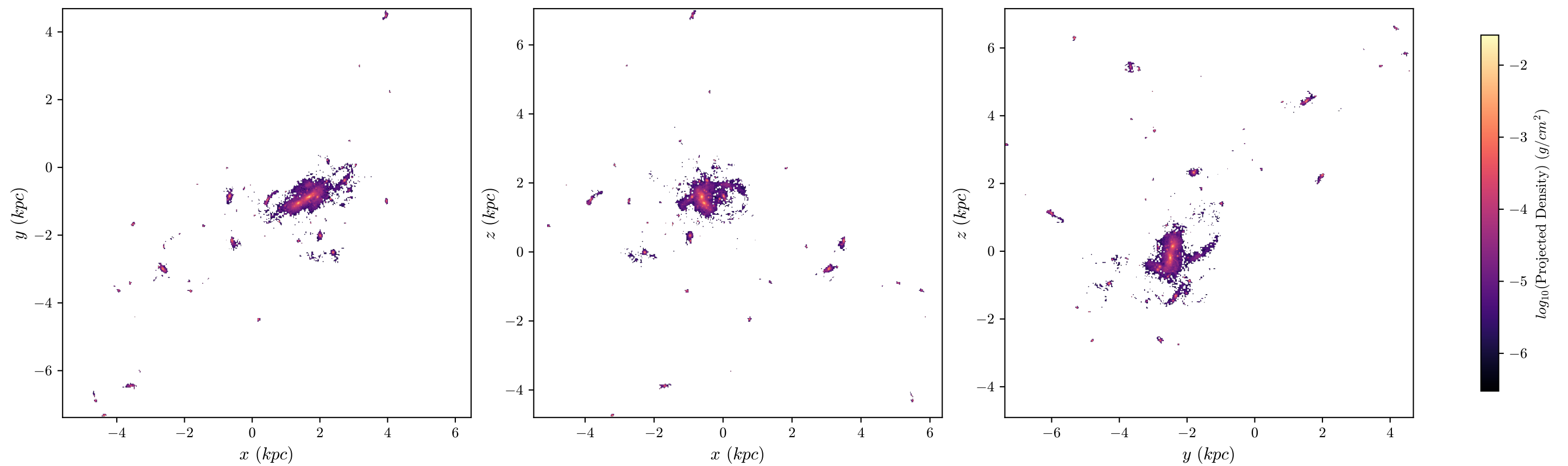
halo8 Stars, z = 3.914 , 512 bins
