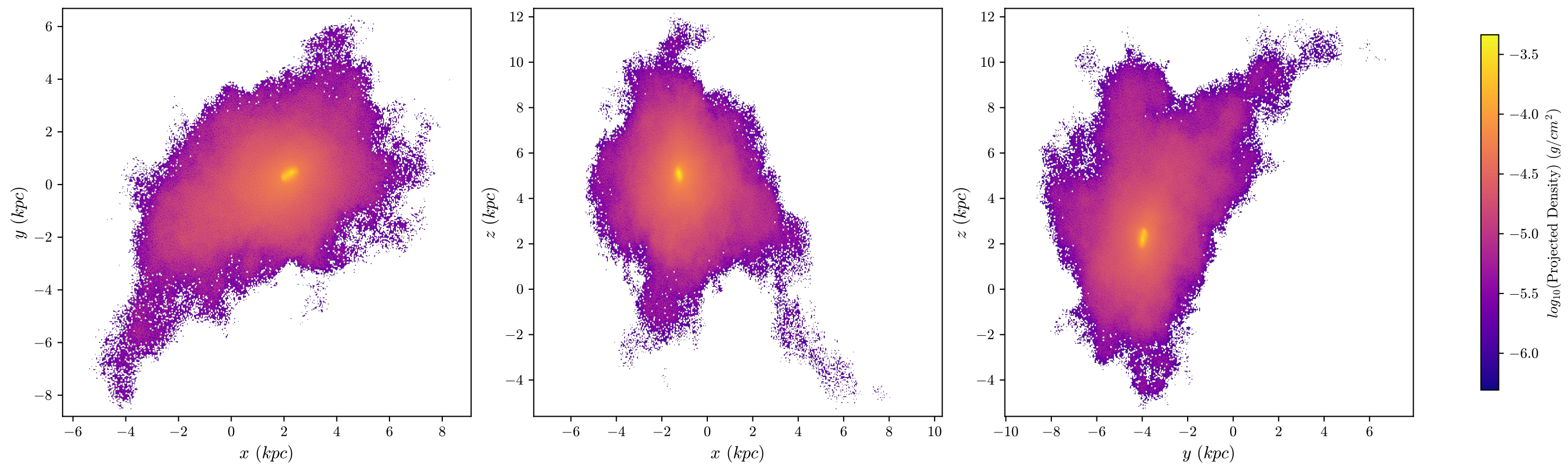
halo8 Dark Matter, z = 3.914 , 512 bins
