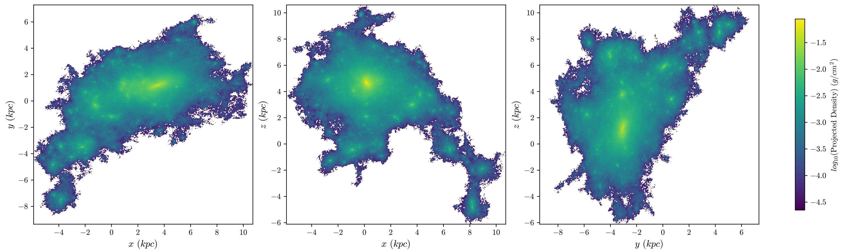
halo8 Stars, z = 3.868 , 512 bins
