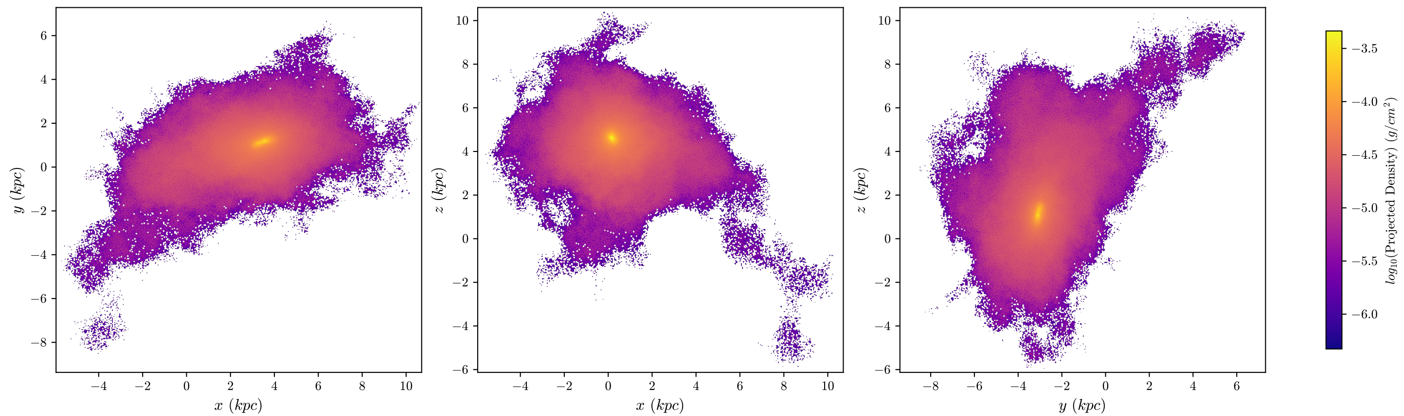
halo8 Dark Matter, z = 3.868 , 512 bins
