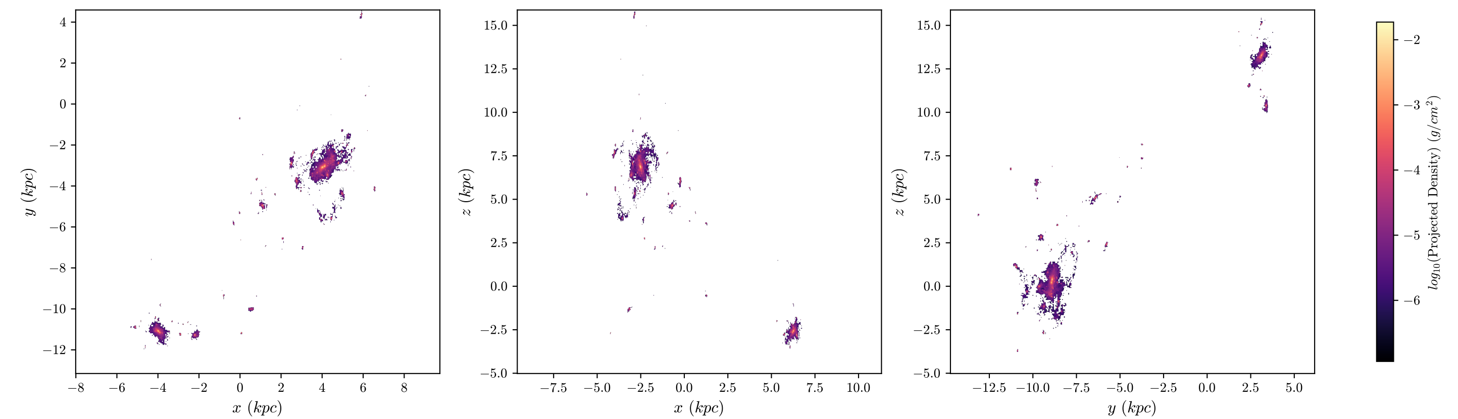
halo8 Stars, z = 3.822 , 512 bins
