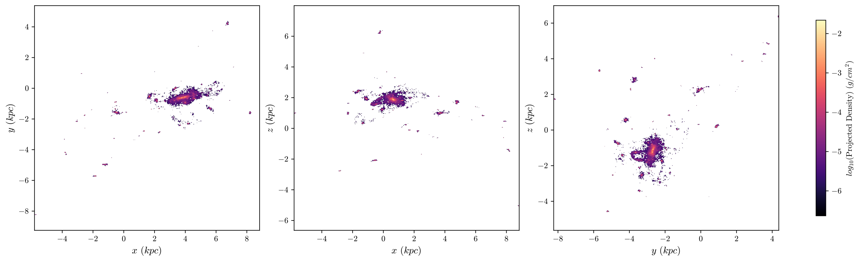
halo8 Stars, z = 3.776 , 512 bins
