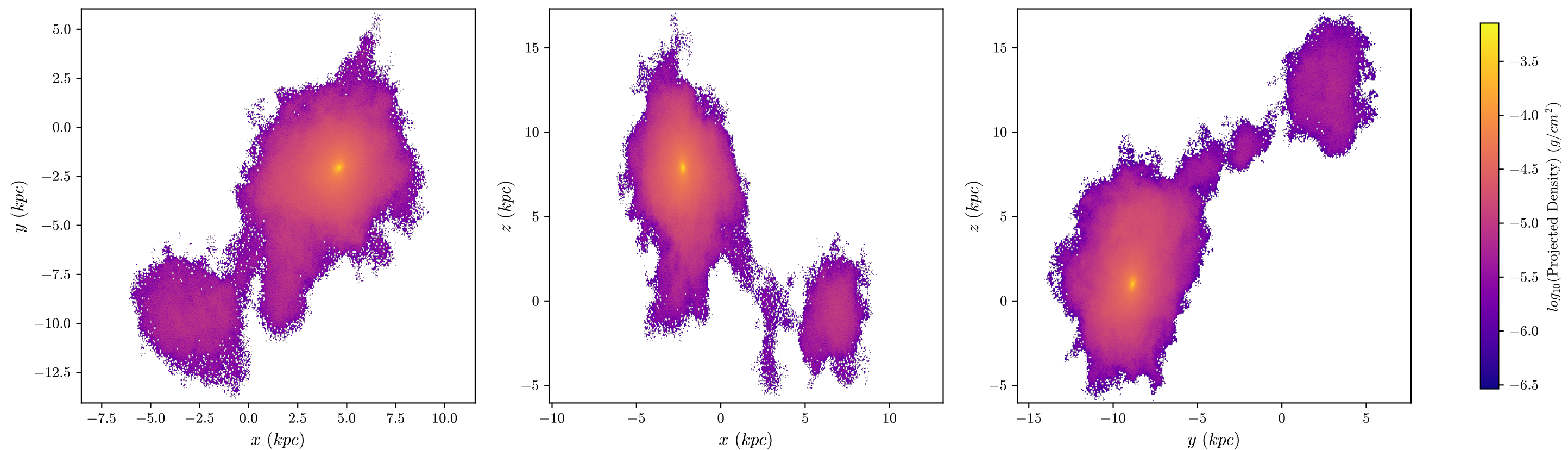
halo8 Dark Matter, z = 3.731 , 512 bins
