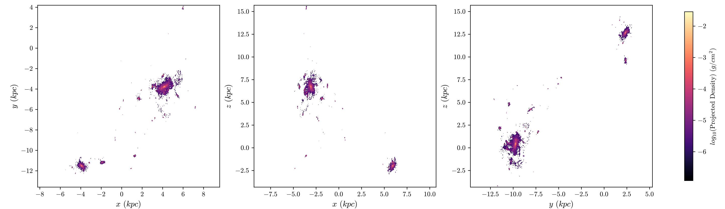
halo8 Stars, z = 3.731 , 512 bins
