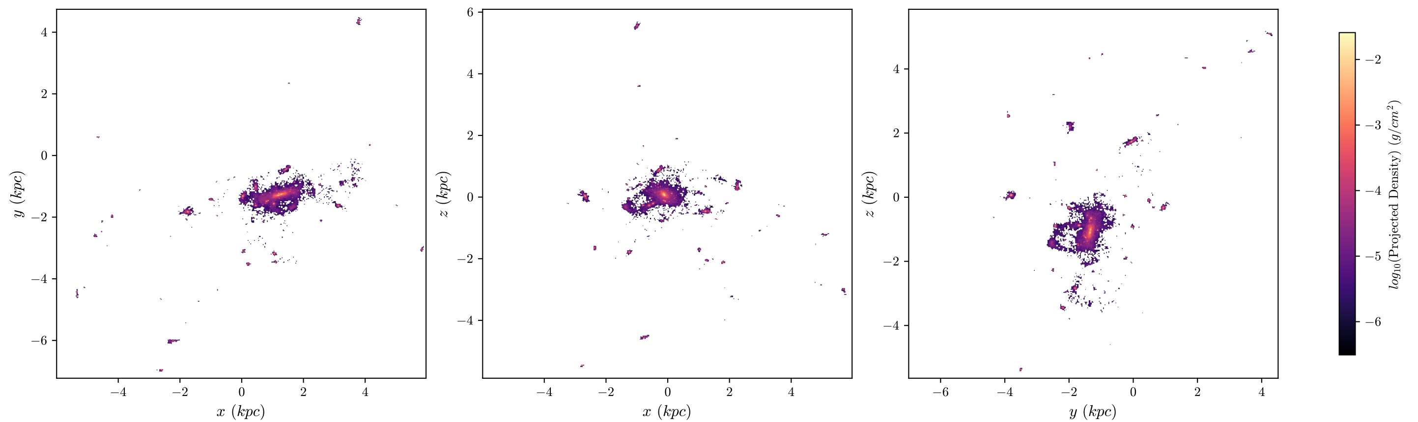
halo8 Stars, z = 3.687 , 512 bins
