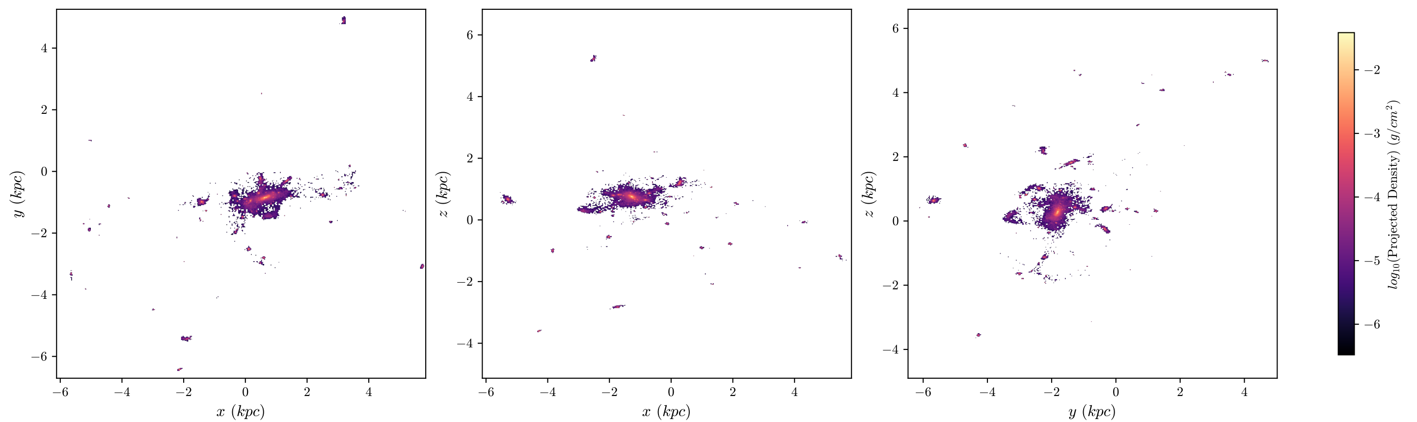
halo8 Stars, z = 3.62 , 512 bins
