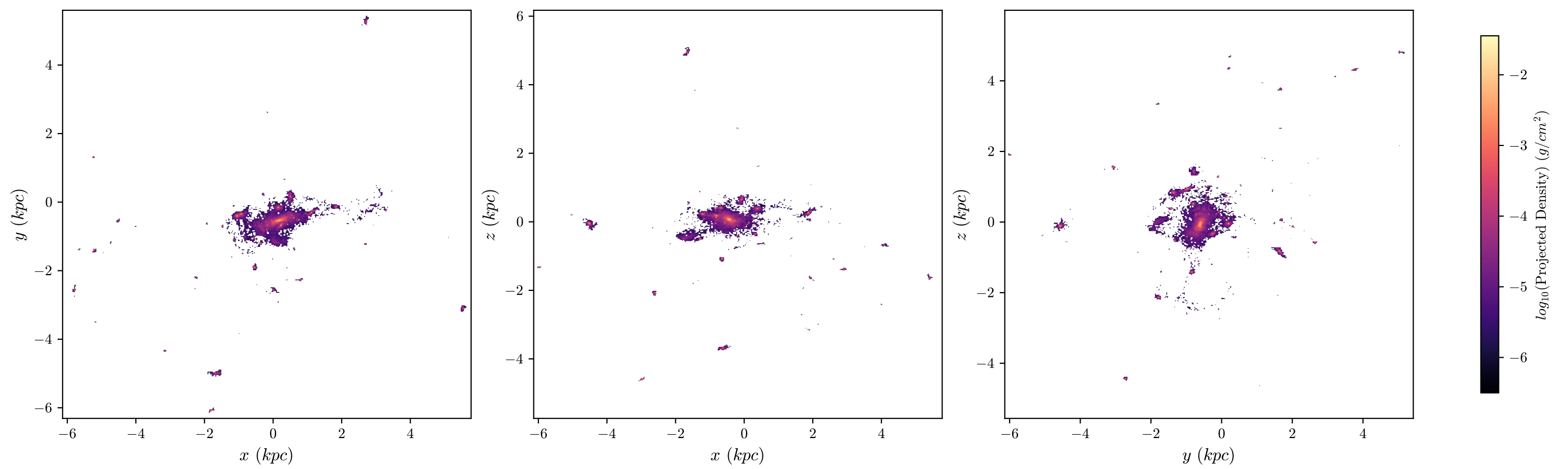
halo8 Stars, z = 3.577 , 512 bins
