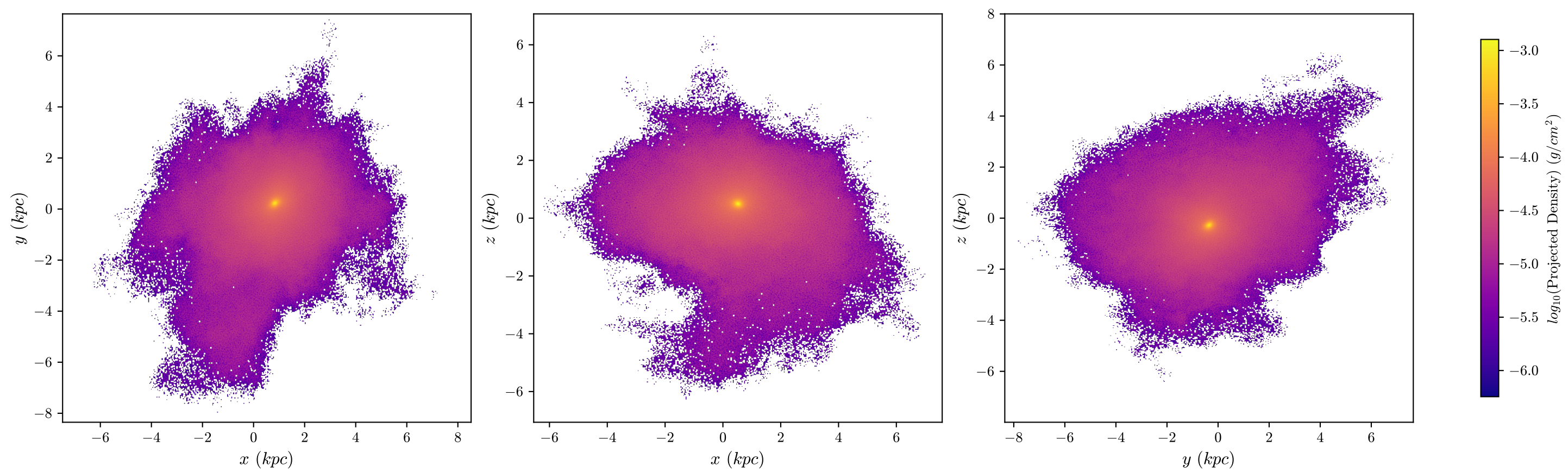
halo8 Dark Matter, z = 3.577 , 512 bins
