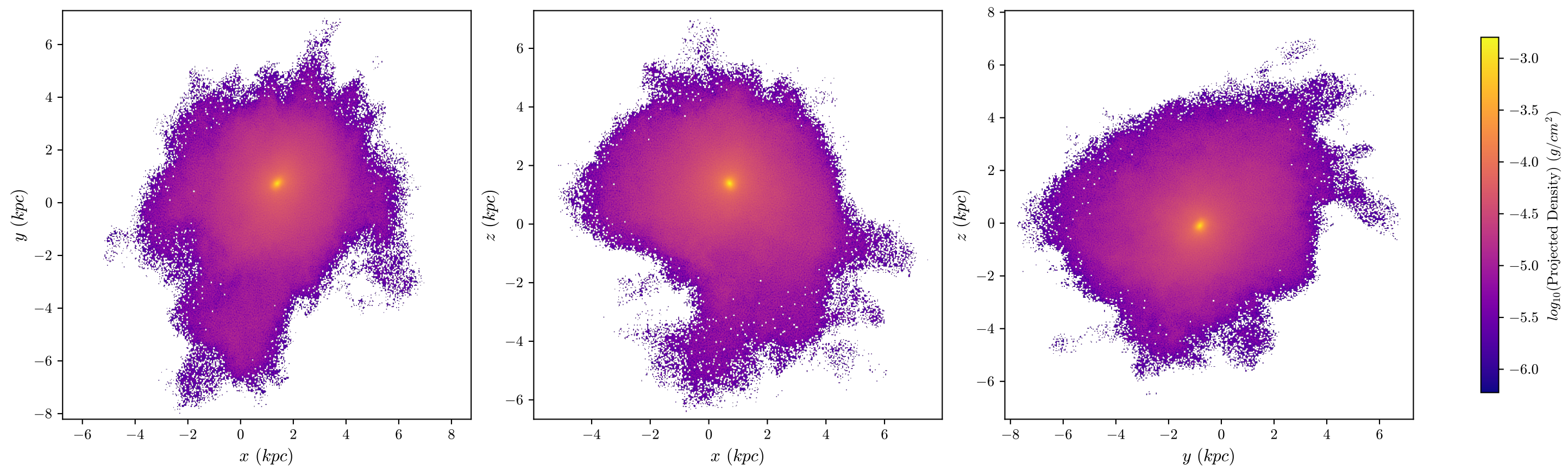
halo8 Dark Matter, z = 3.534 , 512 bins
