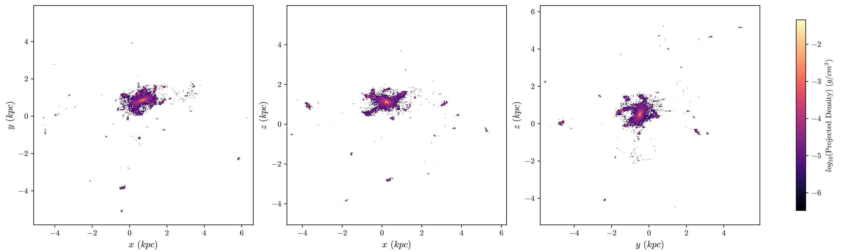
halo8 Stars, z = 3.534 , 512 bins
