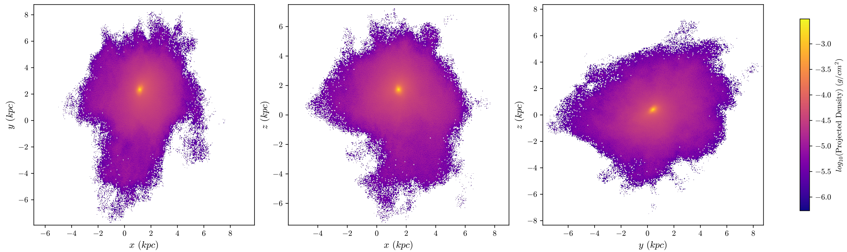
halo8 Dark Matter, z = 3.427 , 512 bins
