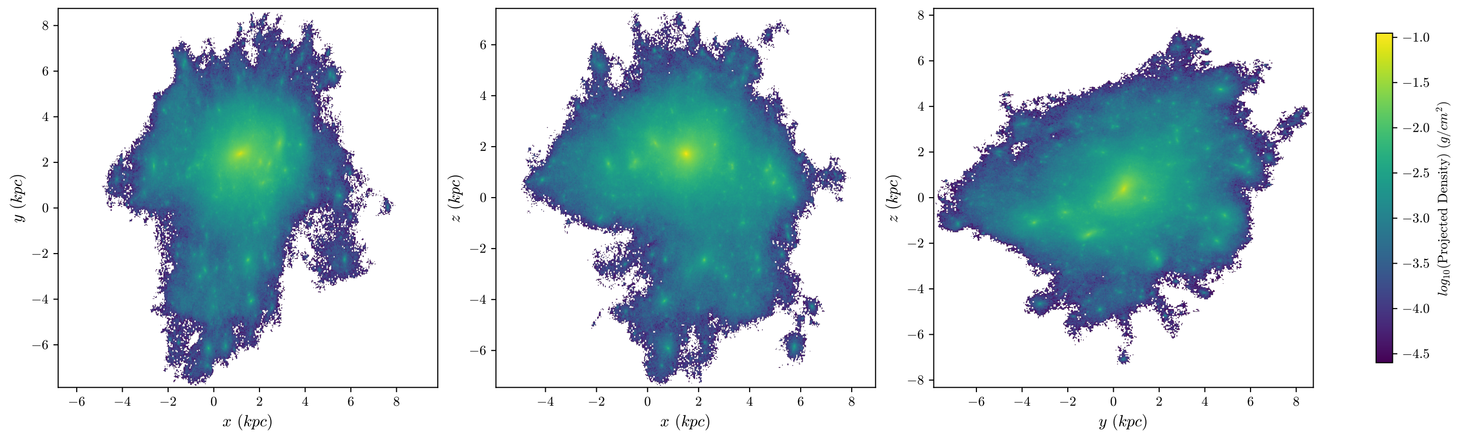
halo8 Stars, z = 3.427 , 512 bins
