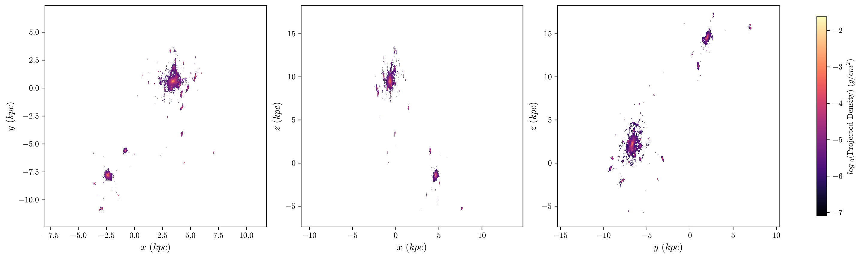
halo8 Stars, z = 3.365 , 512 bins
