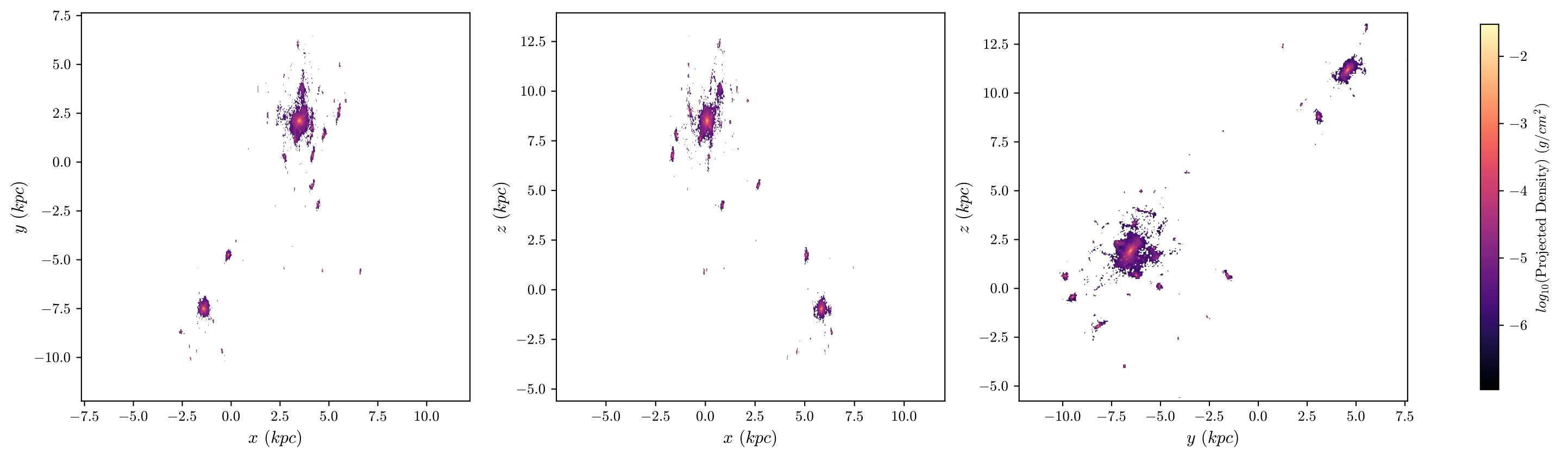
halo8 Stars, z = 3.324 , 512 bins
